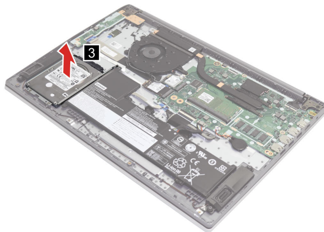
Figure 10. Disconnect the storage drive cable and remove the storage drive with bracket
