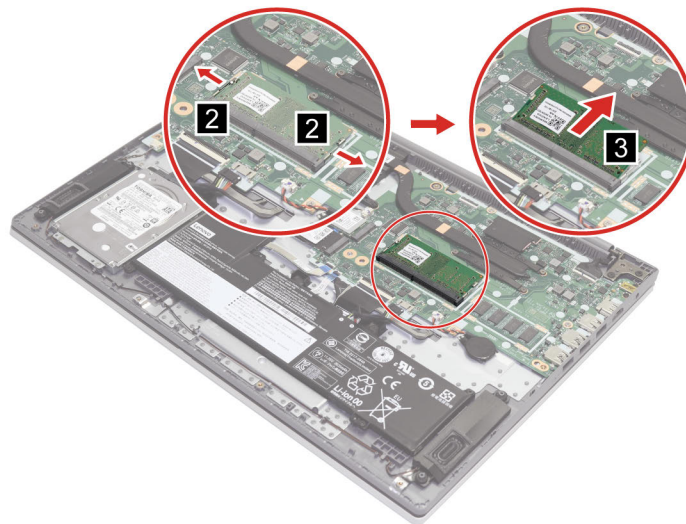
Figure 22. Disengage the latch and slide the memory module out of the slot
