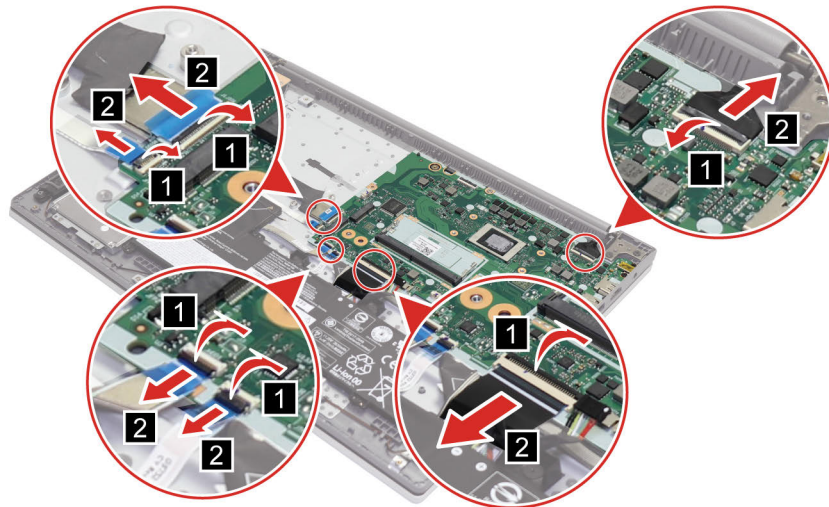
Figure 31. Disconnect cables
