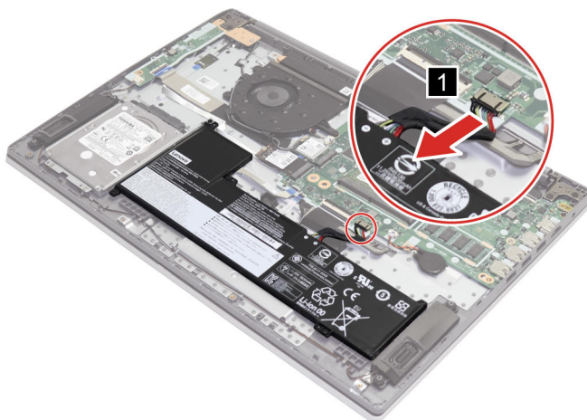
Figure 8. Disconnect the battery pack cable
