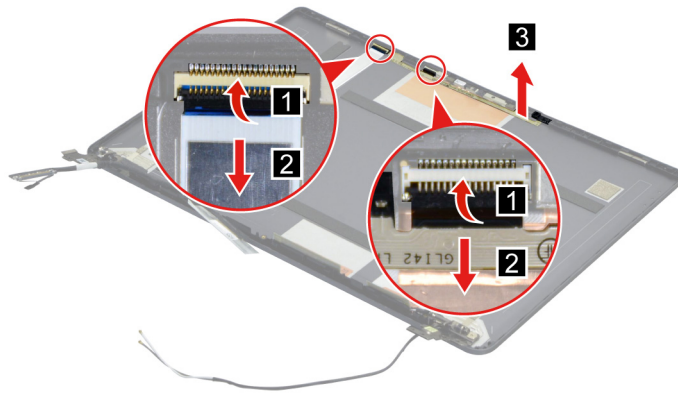
Figure 32. Remove the camera cable
