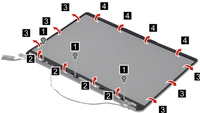
Figure 25. Remove three screws and then remove the LCD bezel
