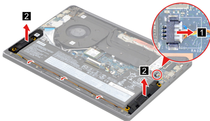
Figure 12. Disconnect the speaker cable from the system board and then release the speaker cable from the cable guide. Remove the speakers carefully.
