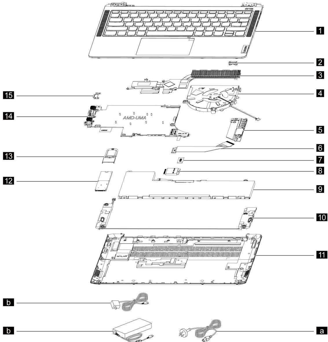
Figure 1. IdeaPad 5 Pro 14ITL6 and IdeaPad 5 Pro 14ACN6 exploded view
