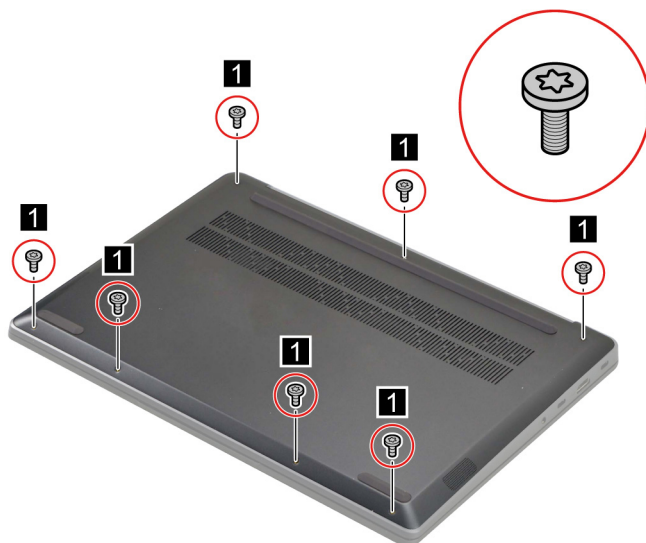
Figure 3. Remove seven screws
