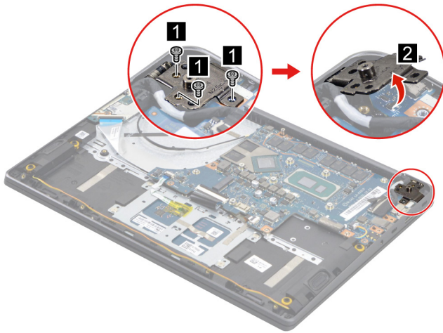
Figure 17. Remove three screws and then open the hinge
