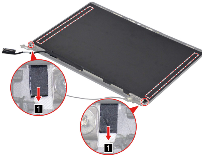
Figure 27. Remove the two pieces of removable tape with tweezers
