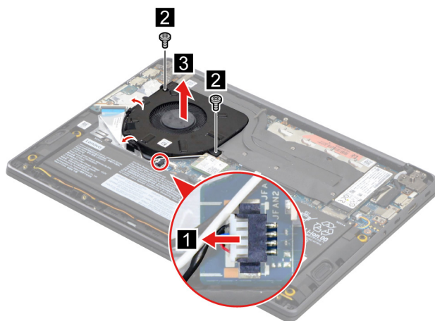
Figure 11. Disconnect the fan cable from the system board and then release the fan cable from the cable guide. Remove two screws and then remove the fan
