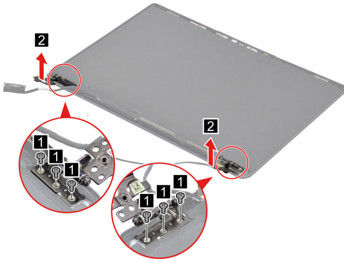
Figure 26. Remove six screws and then remove the hinges
