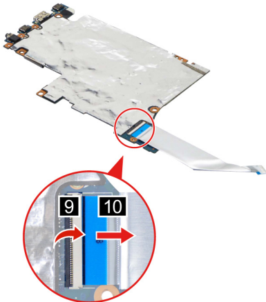
Figure 20. Disconnect the I/O board cable from the system board and then remove the I/O board cable
