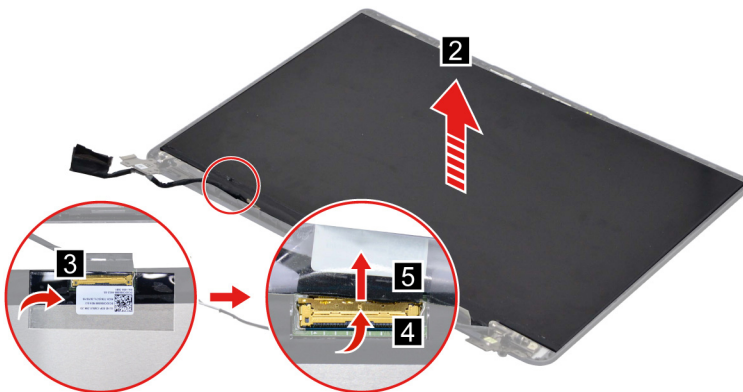
Figure 28. Lift the LCD panel and then disconnect the EDP cable from the LCD panel
