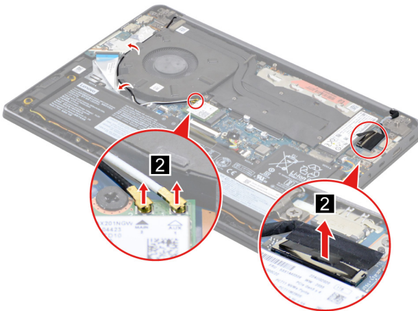
Figure 22. Detach the main and auxiliary antenna cable connectors and then disconnect the EDP cable from the system board
