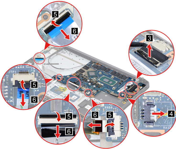
Figure 18. Disconnect cables connected to the system board
