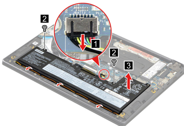
Figure 5. Disconnect the battery pack cable from the system board and then release the battery pack cable from the cable guide. Remove two screws and then remove the battery pack.
