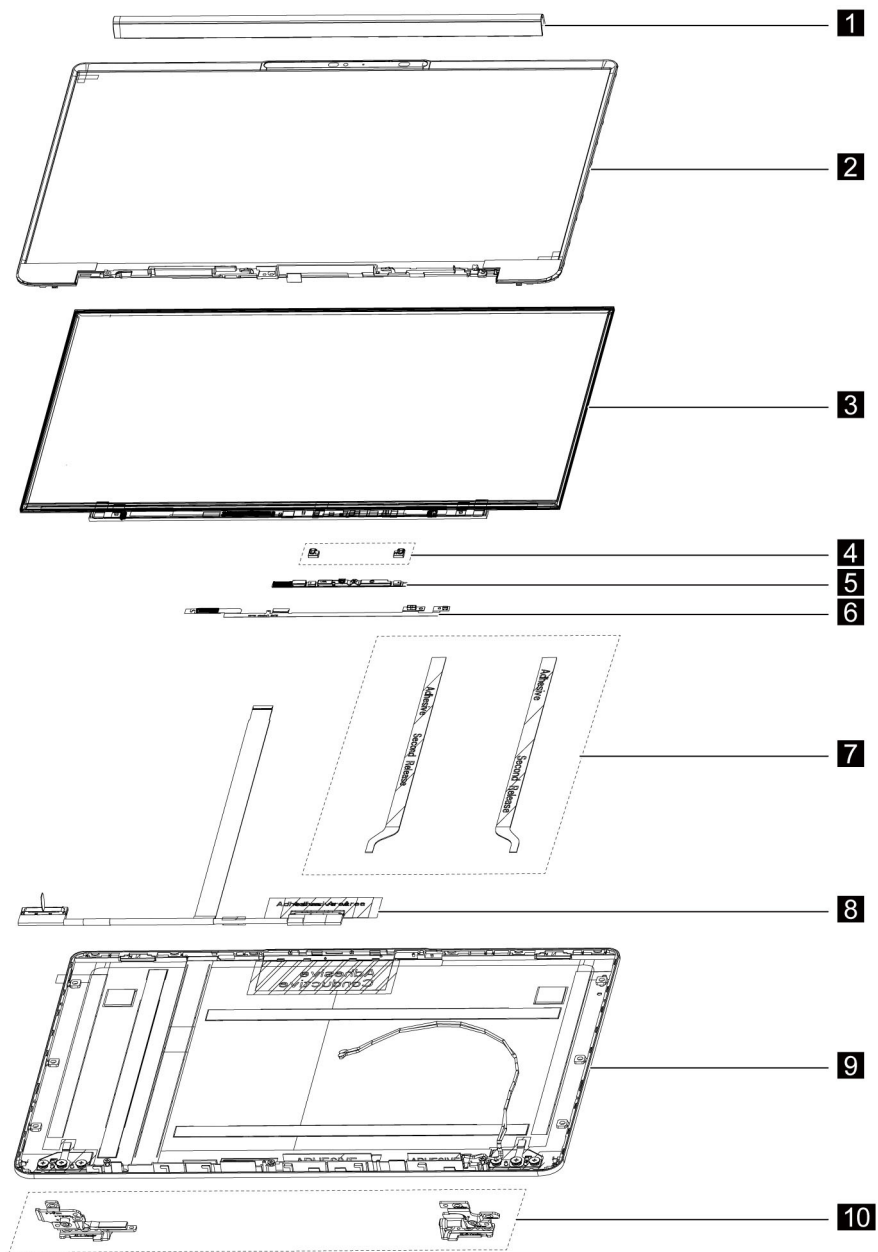
Figure 2. IdeaPad 5 Pro 14ITL6 and IdeaPad 5 Pro 14ACN6 LCD unit - exploded view
