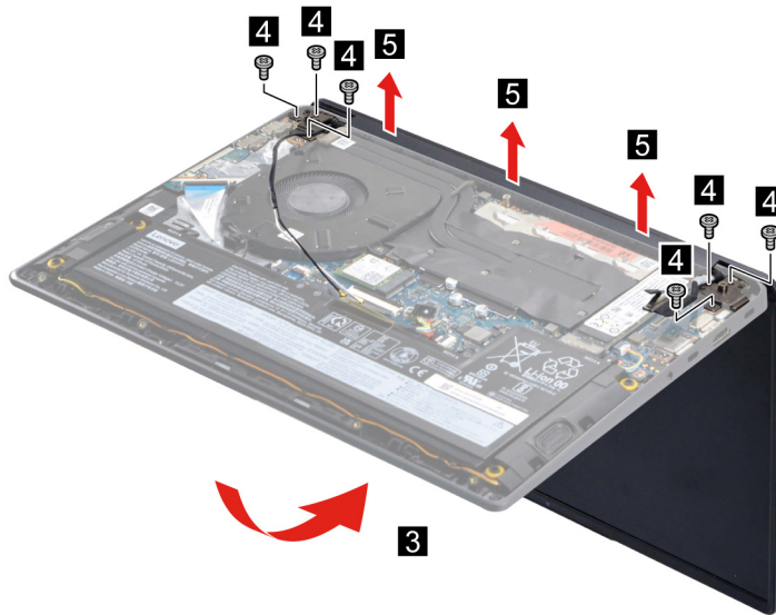
Figure 23. Remove six screws and then remove the LCD unit
