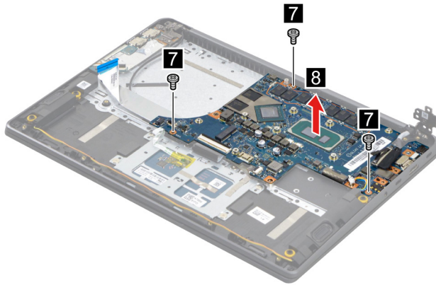
Figure 19. Remove three screws and then remove the system board
