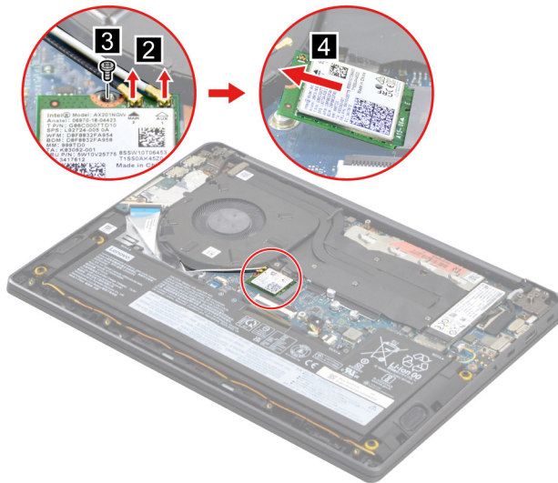
Figure 9. Remove one screw and then remove the Wi-Fi card by pulling it away from the slot
