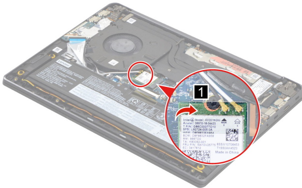
Figure 8. Peel off the WLAN Mylar
