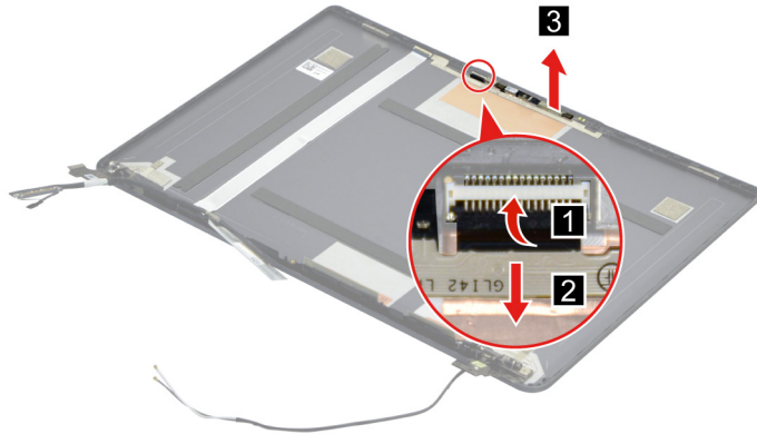
Figure 31. Disconnect the camera cable from the camera board and then remove the camera
