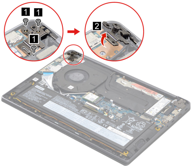
Figure 14. Remove three screws and then open the hinge
