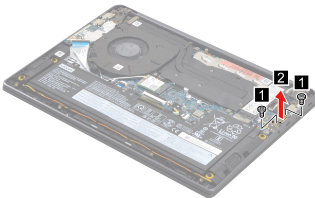
Figure 13. Remove two screws and then remove the USB Type-C bracket
