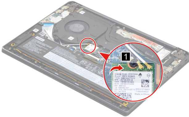
Figure 21. Peel off the WLAN mylar
