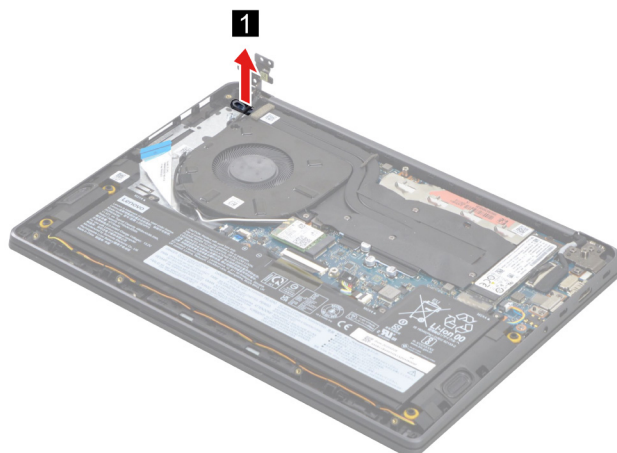
Figure 16. Remove the switch cover carefully
