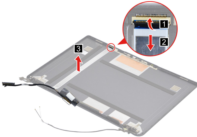
Figure 29. Remove the EDP cable
