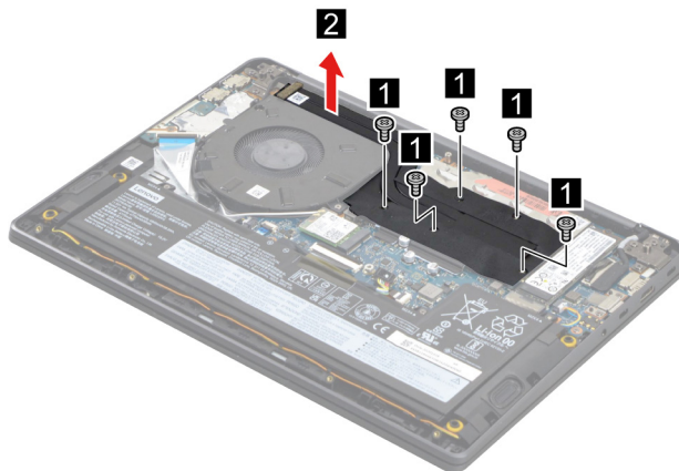
Figure 10. Remove five screws and then remove the heat sink
