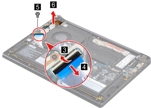
Figure 15. Disconnect the I/O board cable from the I/O board. Remove one screw and then remove the I/O board
