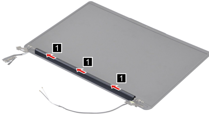
Figure 24. Remove the hinge cover
