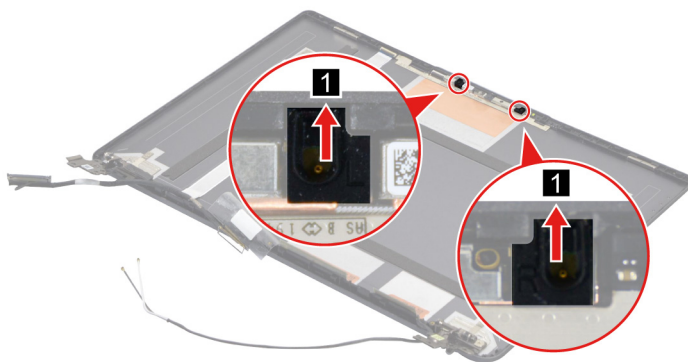
Figure 30. Remove the microphone rubbers
