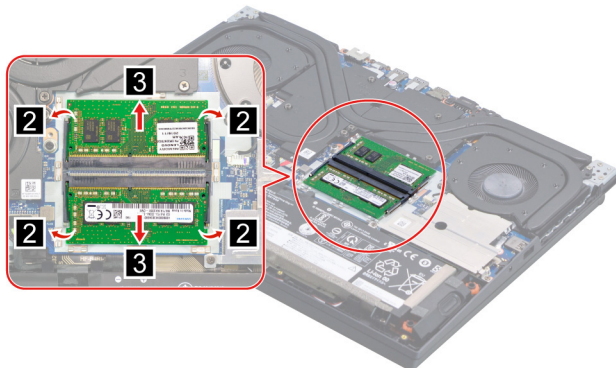
Figure 13. Remove the memory
