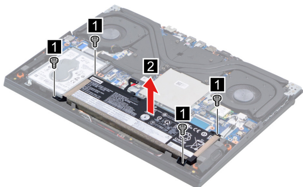
Figure 8. Remove the battery pack
