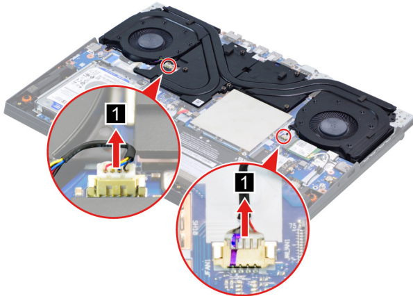
Figure 14. Disconnect the thermal module cables from the system board
