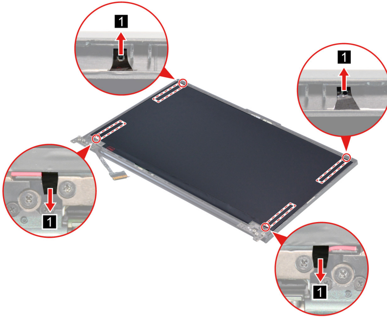
Figure 32. Pull out the pieces of adhesive tape with tweezers
