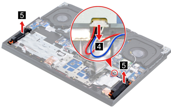
Figure 20. Remove the speakers
