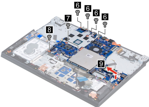
Figure 23. Remove six screws and lift the system board
