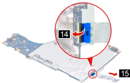
Figure 25. Remove the I/O board cable
