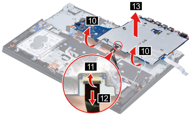
Figure 24. Remove the system board
