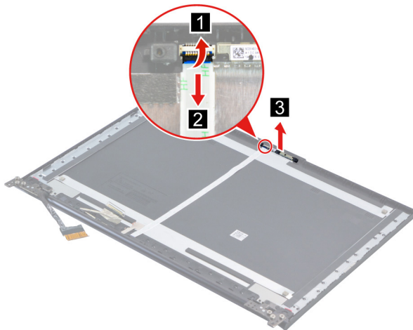
Figure 34. Remove the camera
