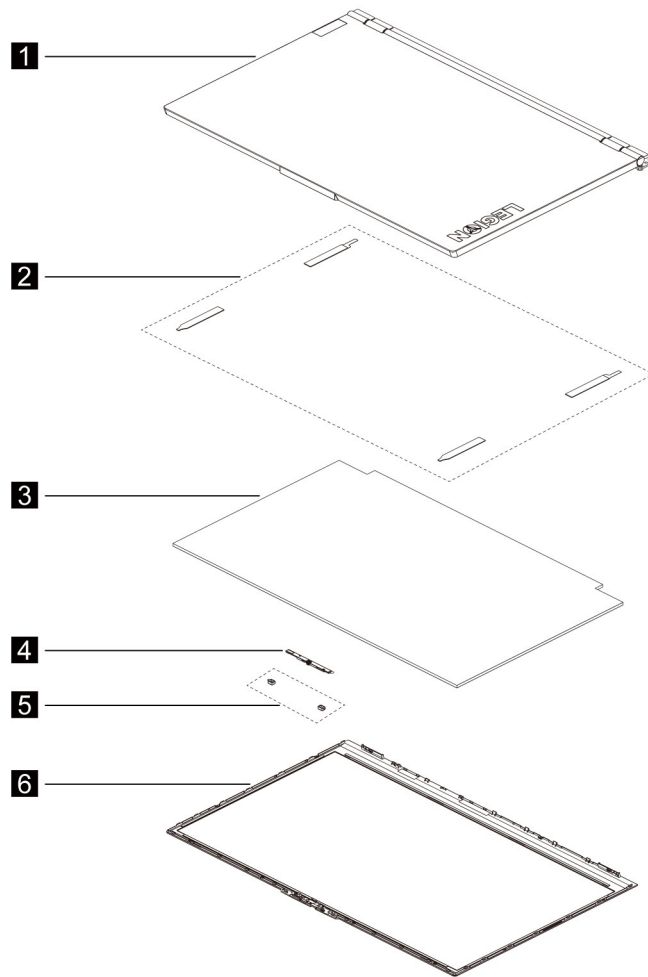
Figure 2. Legion 5 15IMH6 and Lenovo Legion 5 15IMH6 LCD module - exploded view
