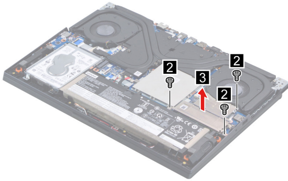
Figure 6. Remove the SSD plate
