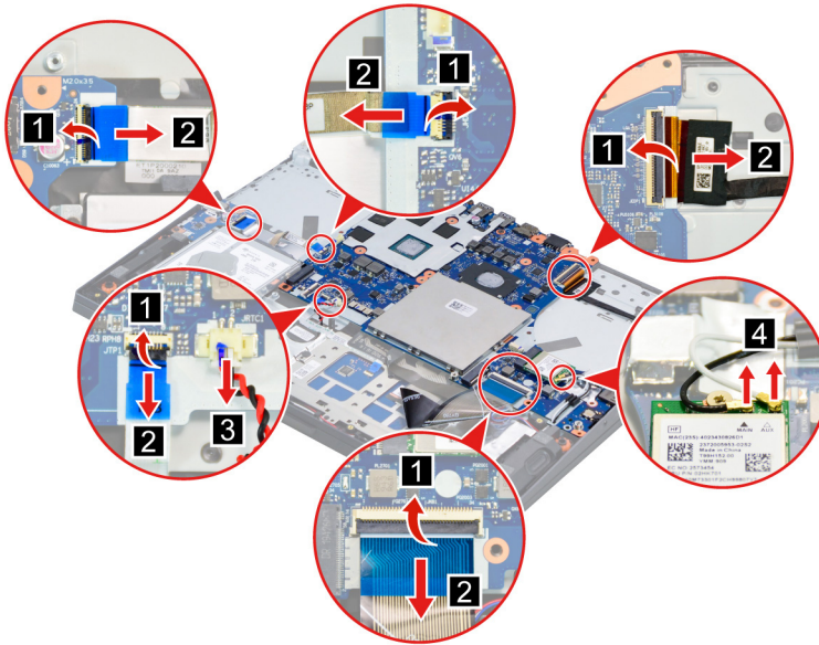
Figure 21. Disconnect cables
