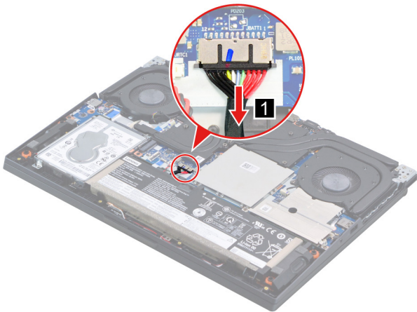
Figure 5. Disconnect the battery cable from the system board
