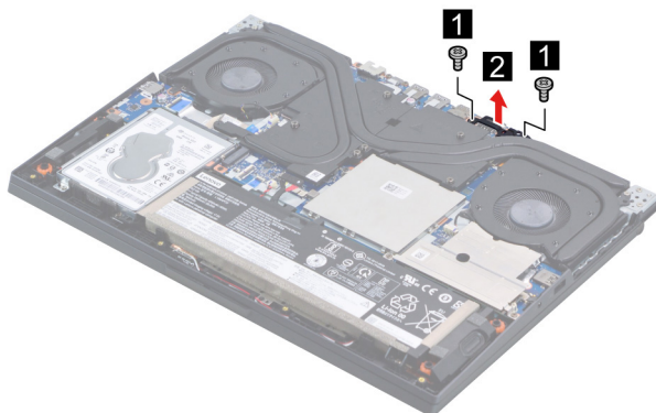
Figure 17. Remove the Kensington lock
