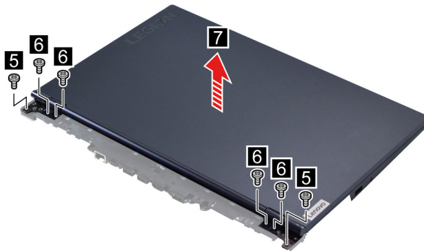
Figure 29. Remove six screws and lift the LCD module
