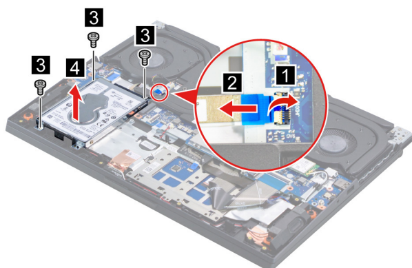
Figure 10. Remove the HDD module
