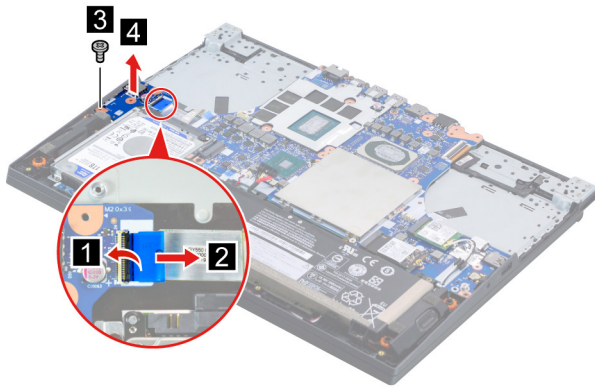
Figure 16. Remove the I/O board
