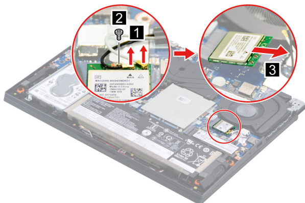
Figure 9. Remove the Wi-Fi card
