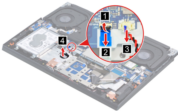
Figure 18. Remove the RTC battery
