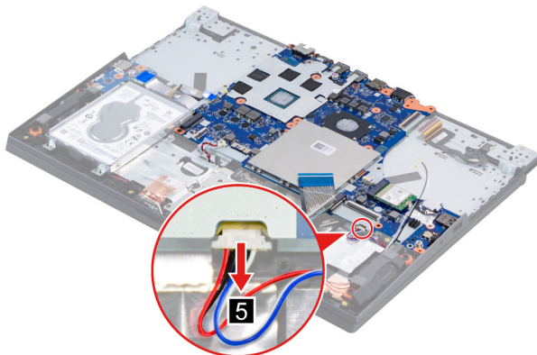
Figure 22. Disconnect the speaker cable from the system board
