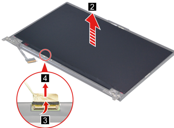
Figure 33. Remove the LCD panel
