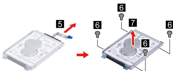
Figure 11. Separate the HDD cable, HDD and the HDD bracket
