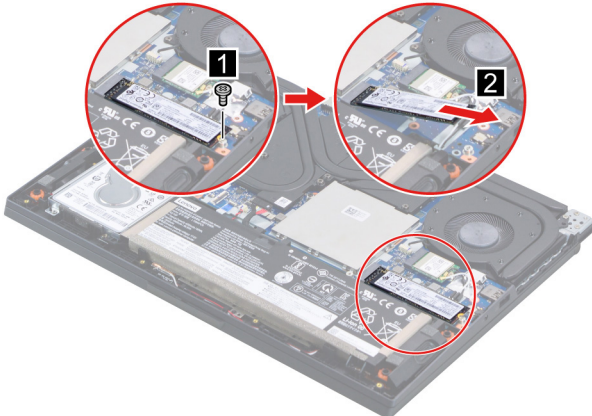
Figure 7. Remove the SSD
