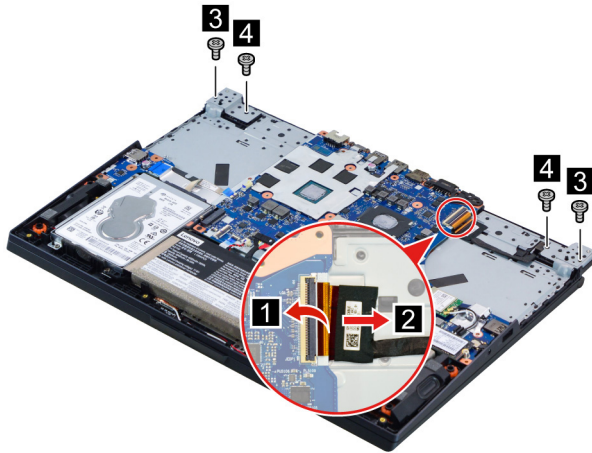
Figure 28. Disconnect the EDP cable from the system board and remove four screws
