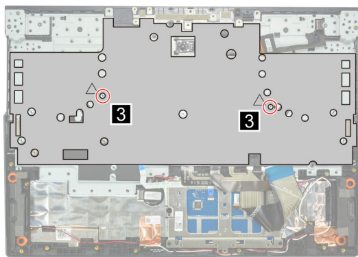
Figure 37. Attach the keyboard bracket mylar
