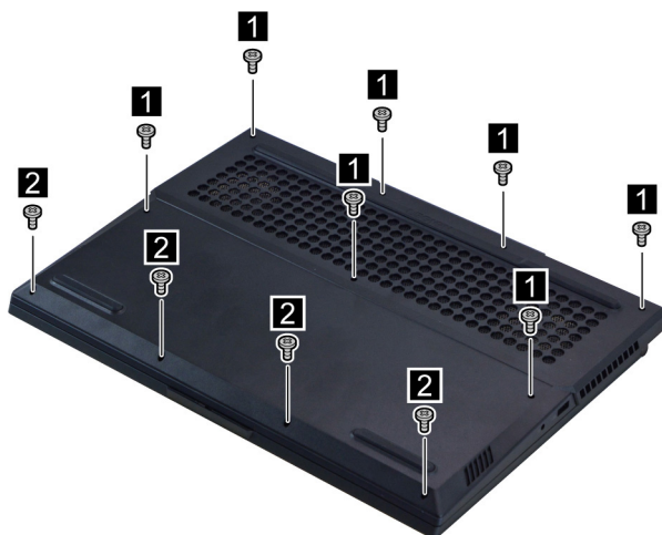
Figure 3. Remove eleven screws
