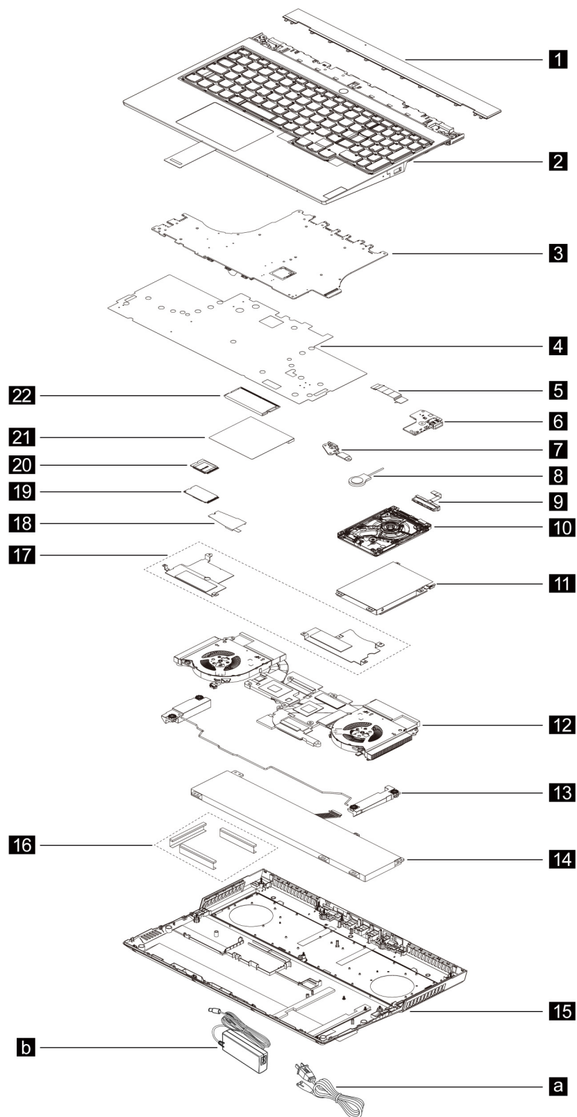
Figure 1. Legion 5 15IMH6 and Lenovo Legion 5 15IMH6 exploded view
