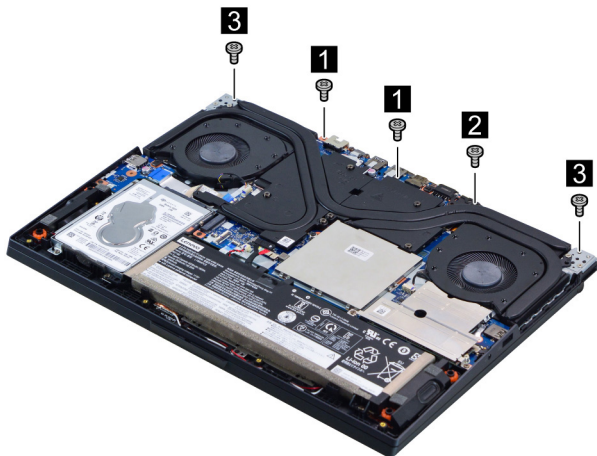
Figure 26. Remove five screws
