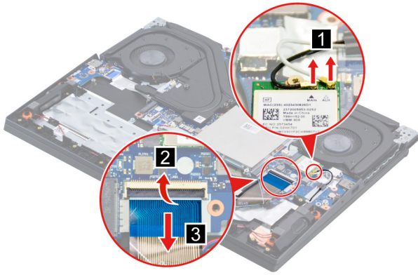
Figure 19. Detach the cables
