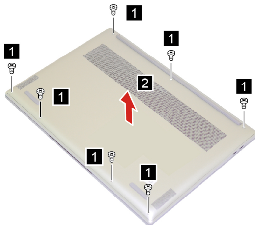
Figure 5. Remove seven screws
