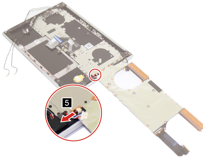
Figure 27. Disconnect the coin-cell battery cable
