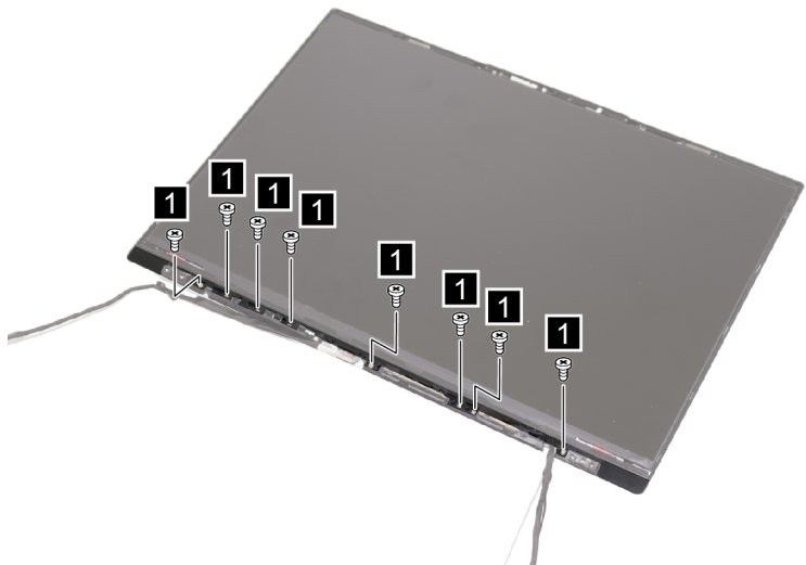
Figure 45. Remove eight screws
