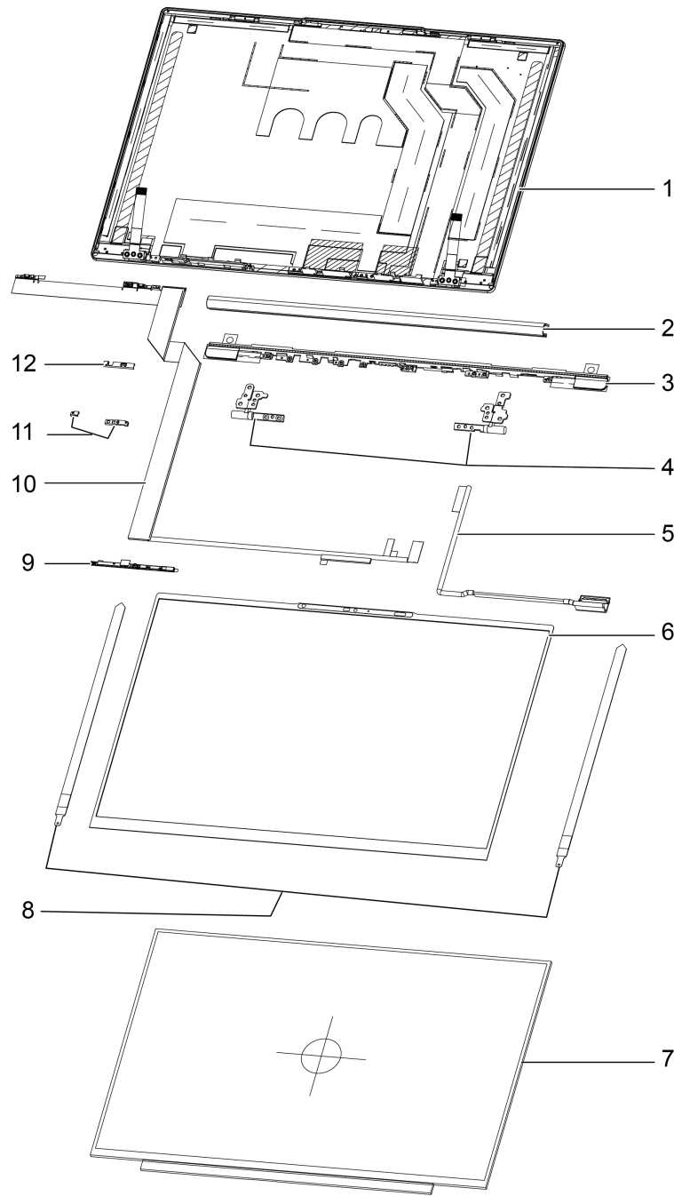
Figure 4. LCD exploded view (for mylar models)
