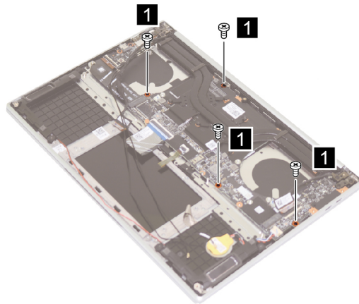
Figure 24. Remove four screws
