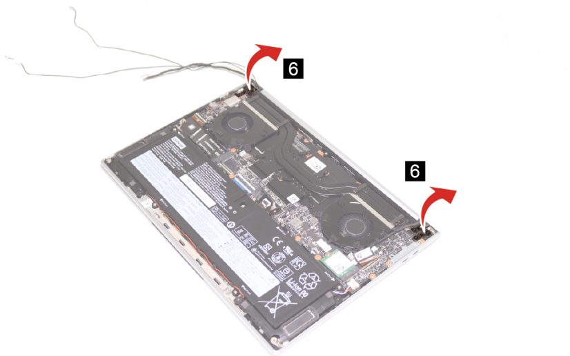
Figure 30. Open the hinges
