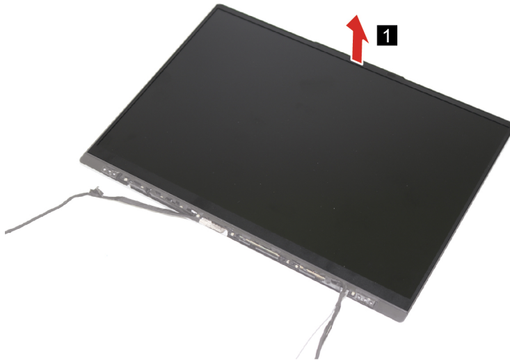
Figure 52. Remove the LCD bezel
