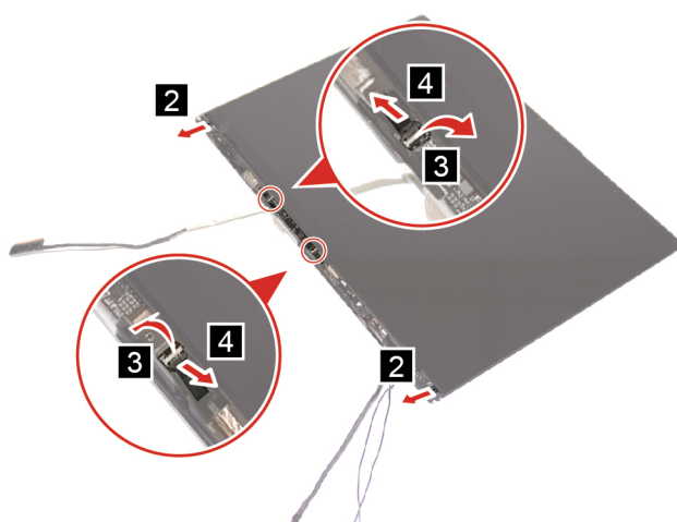
Figure 48. Pull out two adhesive and disconnect the PMIC board connector
