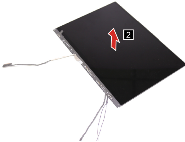
Figure 54. Lift the LCD panel
