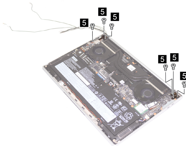
Figure 29. Remove six screws
