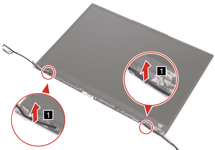
Figure 38. Remove the hinge cover
