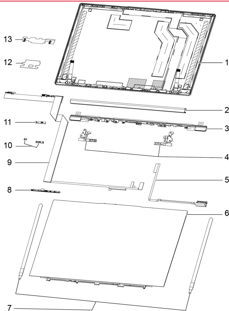
Figure 3. OLED exploded view (for glass models)
