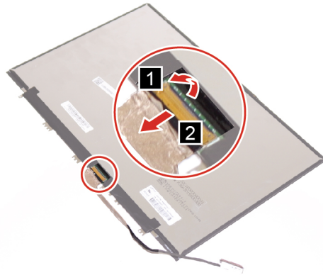
Figure 55. Remove the EDP cable
