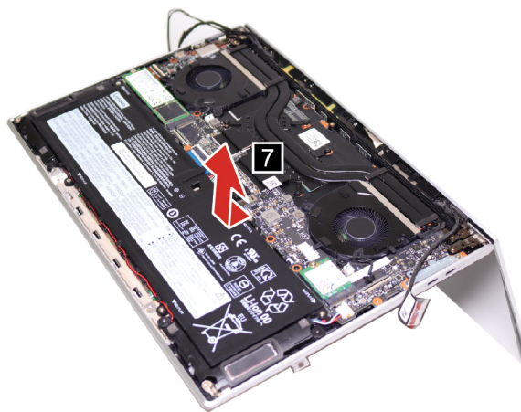
Figure 31. Remove the upper case
