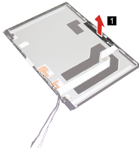
Figure 59. Remove the camera and cable
