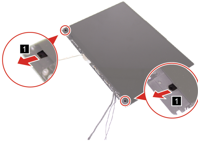
Figure 50. Pull out two adhesive
