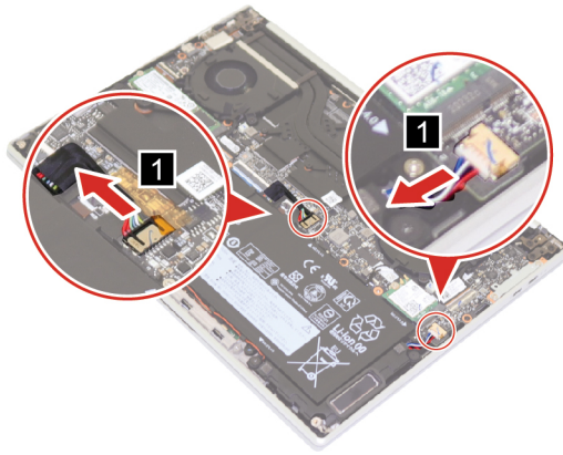
Figure 22. Disconnect cables
