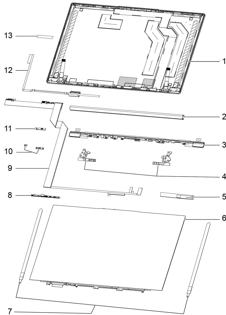
Figure 2. LCD exploded view (for glass models)
