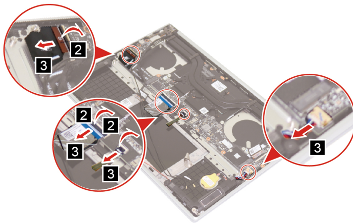
Figure 25. Disconnect all cables
