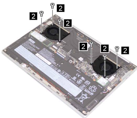
Figure 14. Remove six screws
