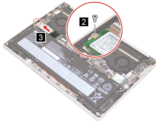
Figure 9. Remove the solid-state drive
