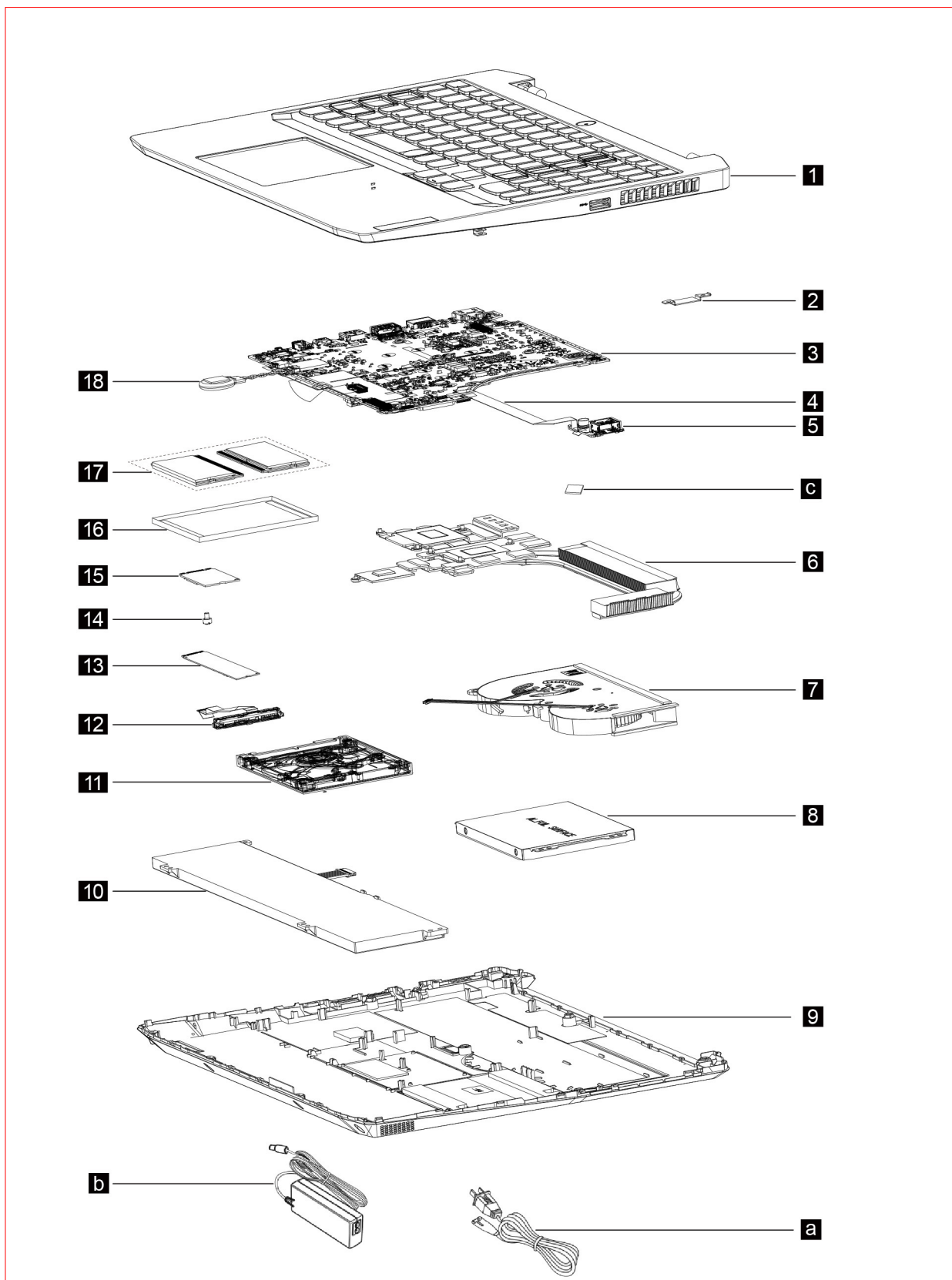
Figure 1. IdeaPad Gaming 3 (15", 05) exploded view
