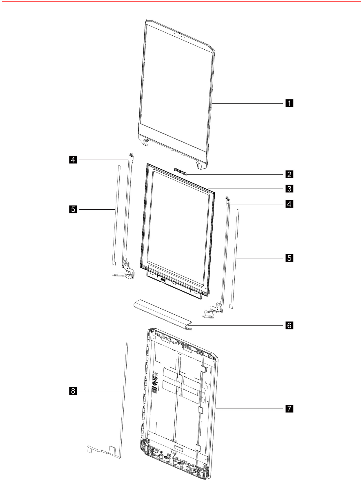
Figure 2. IdeaPad Gaming 3 (15", 05) LCD module - exploded view
