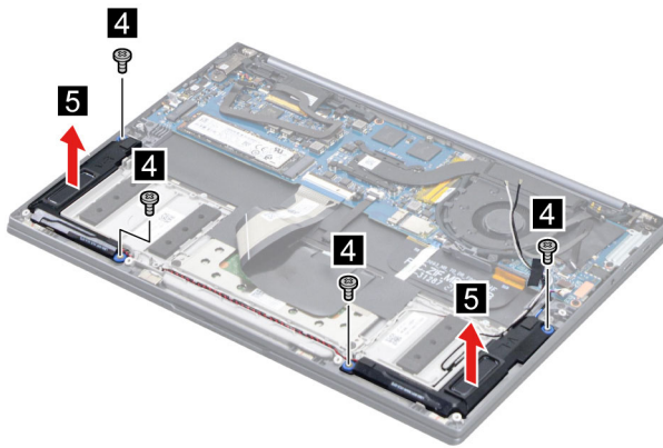
Figure 23. Remove four screws and remove the speakers
