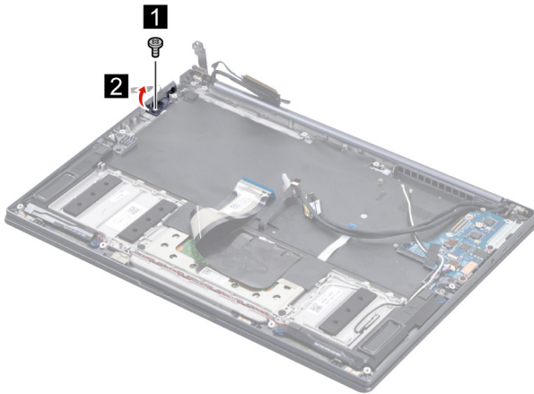
Figure 42. Remove one screw and pry up the fingerprint board holder
