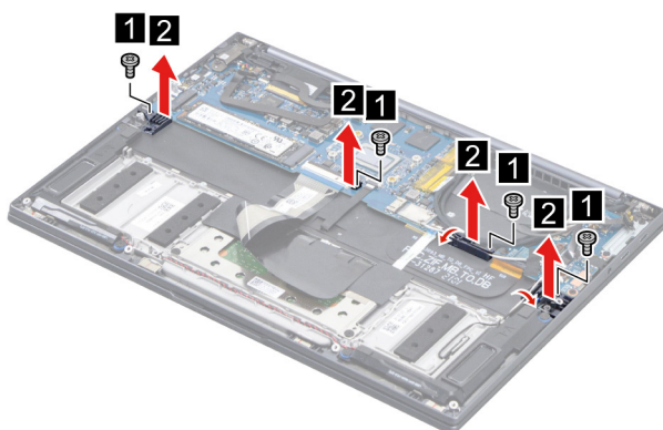
Figure 30. Remove four screws and remove the brackets
