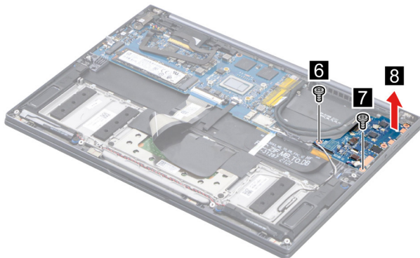
Figure 33. Remove the USB board
