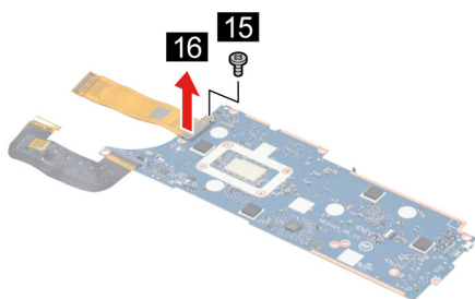
Figure 38. Remove the USB board cable bracket 2
