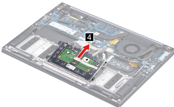
Figure 29. Remove the touchpad
