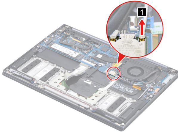
Figure 25. Detach one of the antenna cable connector
