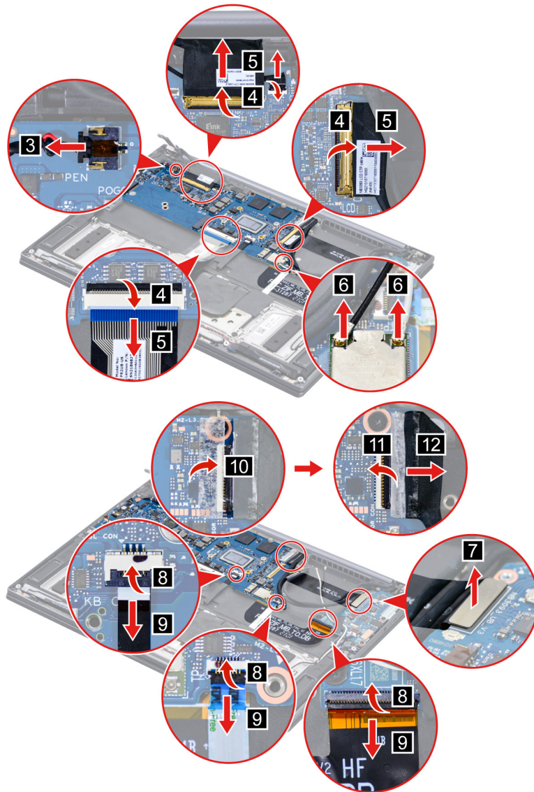
Figure 35. Disconnect cables connected to the system board and disconnect the USB cables from the USB board
