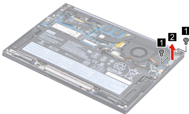
Figure 15. Remove two screws and remove the Type C bracket
