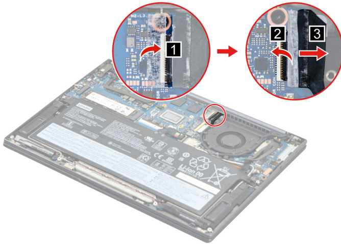
Figure 44. Peel off the tape and disconnect the EDP cable from the system board
