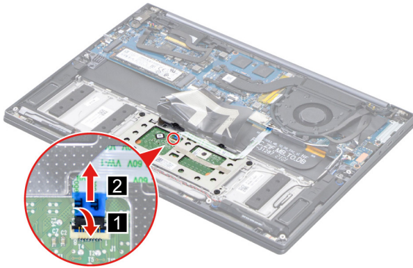
Figure 27. Disconnect the touchpad cable from the touchpad
