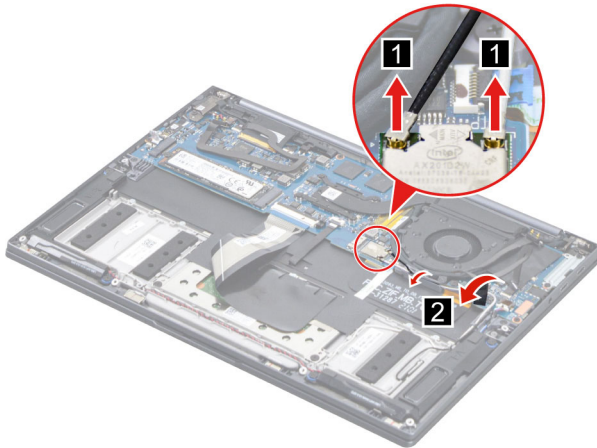
Figure 21. Detach the main and auxiliary antenna cable connectors and release the antenna cables
