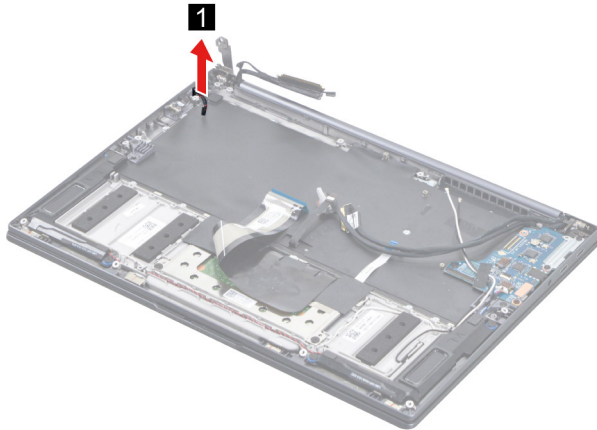
Figure 41. Remove the pen charger cable
