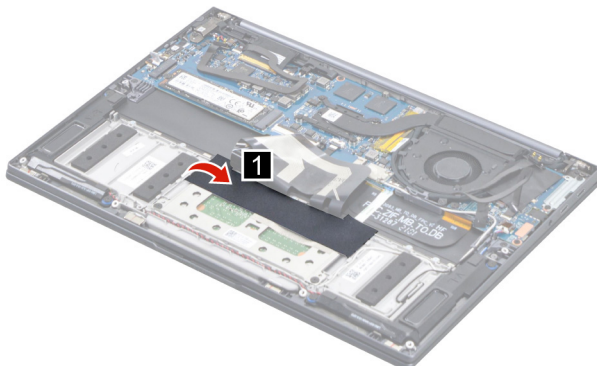
Figure 24. Remove the touchpad mylar
