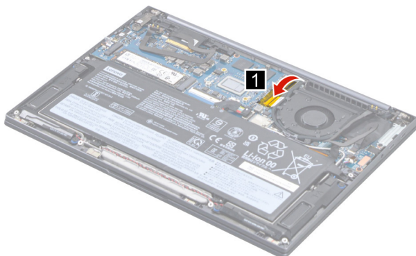
Figure 17. Peel off the golden mylar
