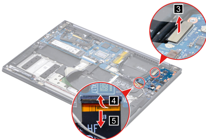
Figure 32. Disconnect cables connected to the USB board
