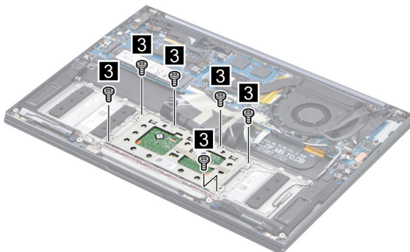
Figure 28. Remove six screws
