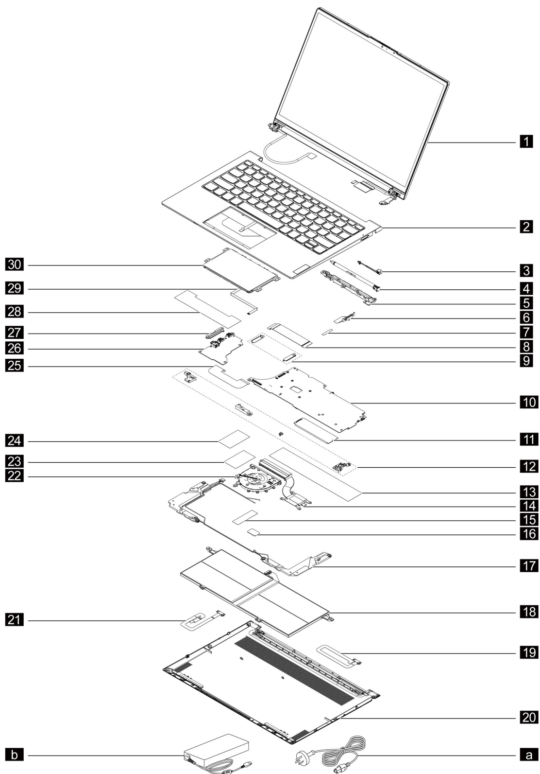
Figure 1. ThinkBook Plus G2 ITG exploded view
