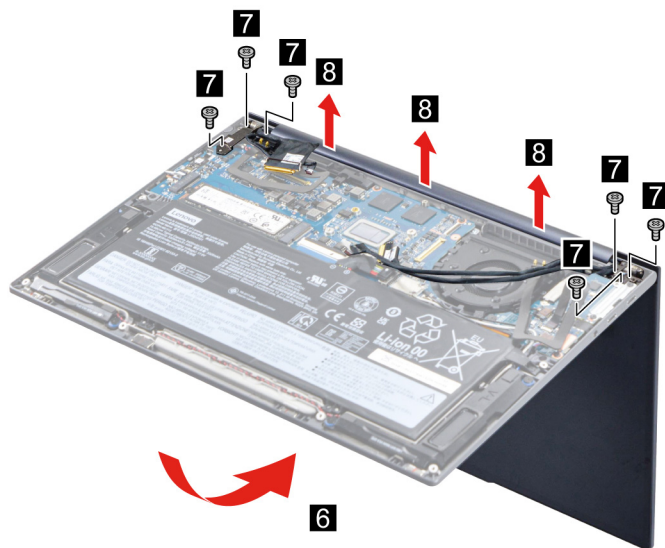
Figure 46. Remove the LCD module
