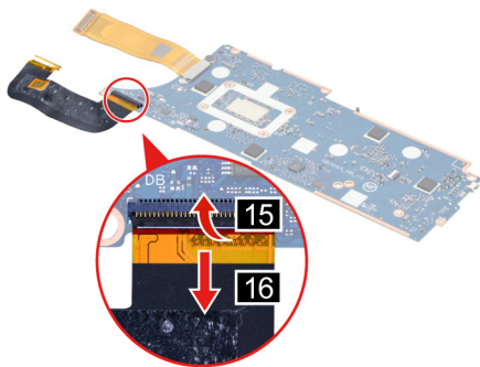
Figure 37. Remove the USB board cable (61 pin)
