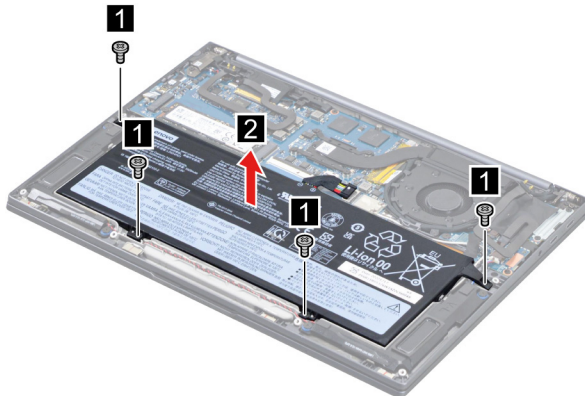
Figure 9. Remove four screws and remove the battery pack
