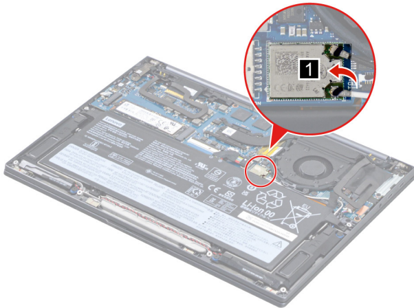
Figure 12. Remove the Wi-Fi card mylar
