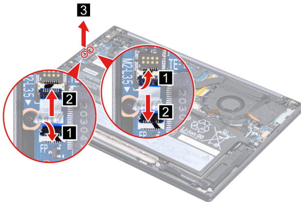
Figure 13. Remove the fingerprint board cable
