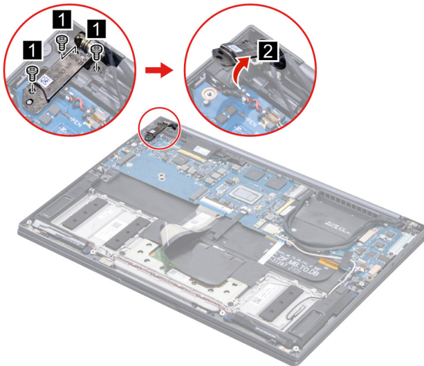
Figure 34. Remove three screws and open the hinge
