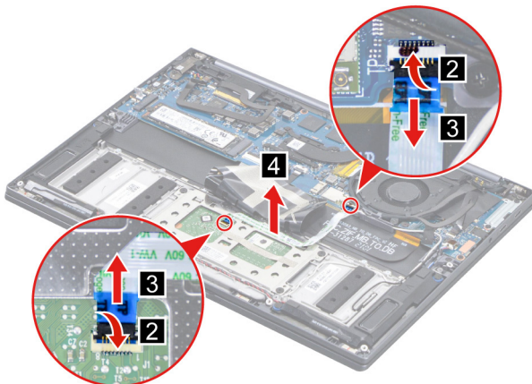
Figure 26. Remove the touchpad cable
