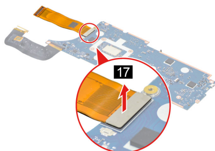
Figure 39. Remove the USB board cable (62 pin)
