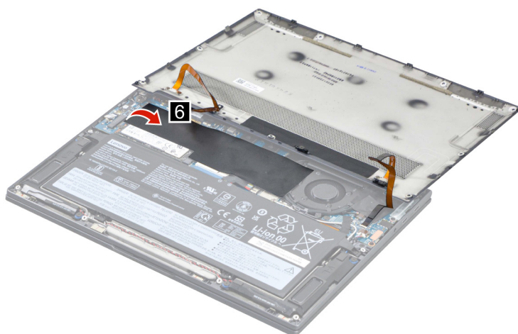
Figure 5. Peel off the system board mylar
