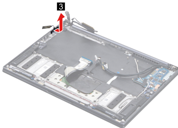
Figure 43. Remove the fingerprint board
