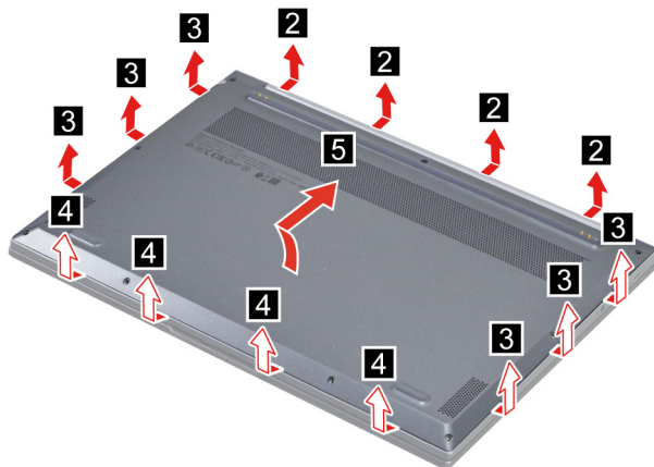
Figure 4. Pry up the latches and open the lower case
