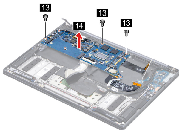
Figure 36. Remove the system board module
