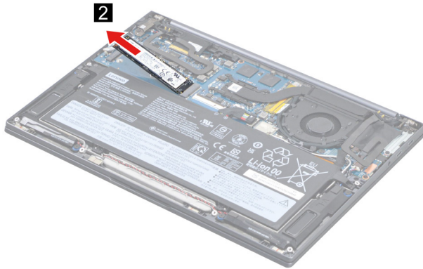
Figure 11. Remove the SSD
