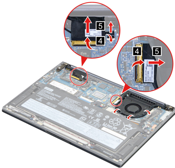
Figure 45. Disconnect the two cables and release the cable from the cable guide
