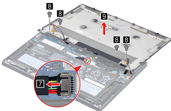
Figure 6. Remove four screws and remove the lower case
