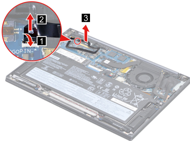
Figure 7. Remove the pogo pin cable (left)
