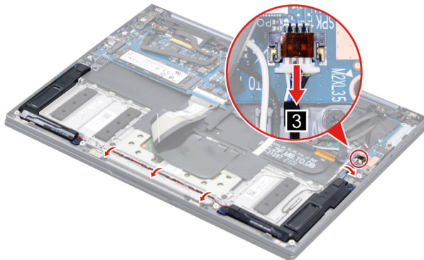
Figure 22. Detach the speaker cable connector and release cables
