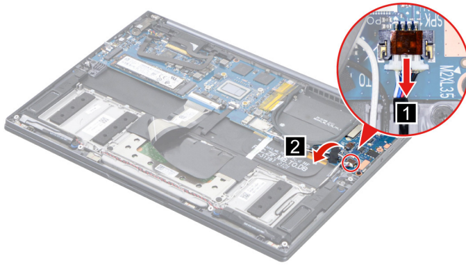
Figure 31. Detach the speaker cable connector and peel off the tape
