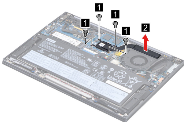
Figure 16. Remove four screws and remove the heat sink
