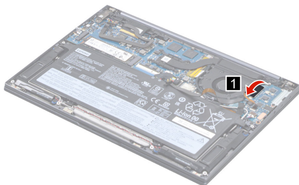
Figure 19. Peel off the tape
