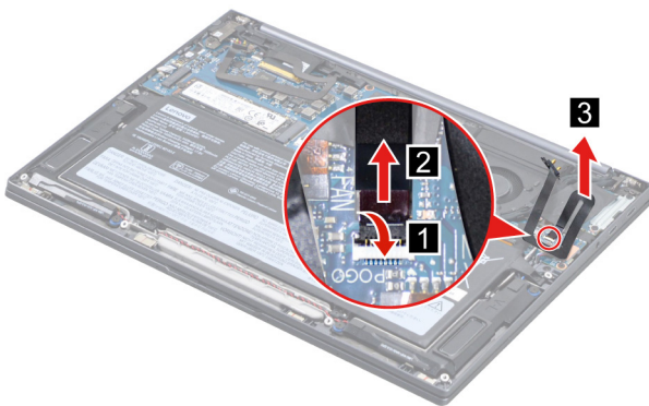
Figure 8. Remove the pogo pin cable (right)
