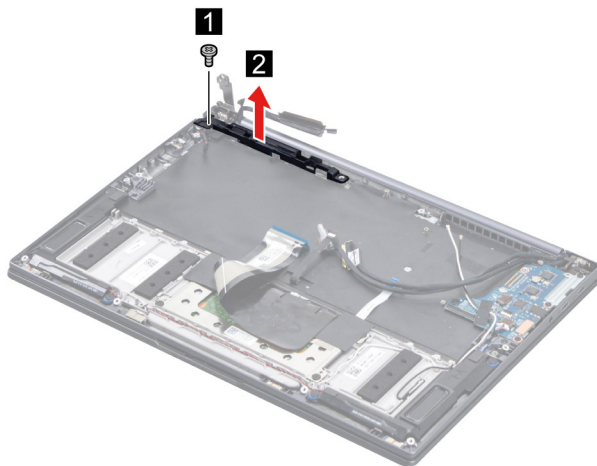
Figure 40. Remove one screw and remove the pen holder
