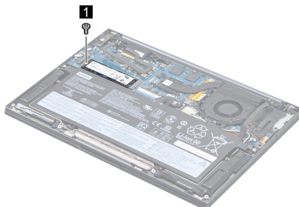
Figure 10. Remove one screw
