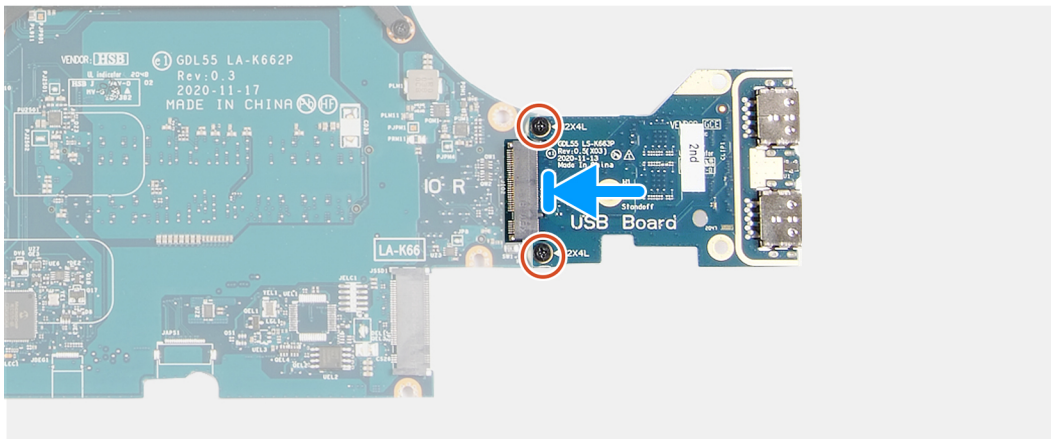
2x M2x4
