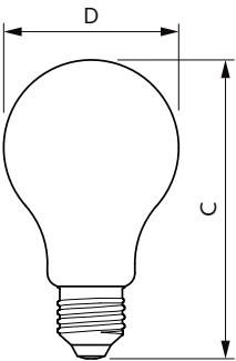
A67 220-240V 120W 2000lm 2700K E27 ND CL
