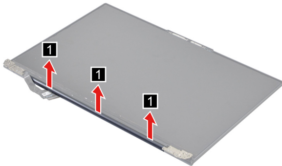
Figure 37. Remove the hinge cover
