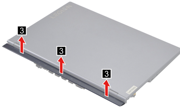
Figure 30. Remove the strip cover
