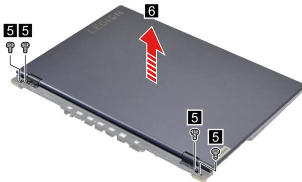
Figure 33. Remove four screws and then lift the LCD module
