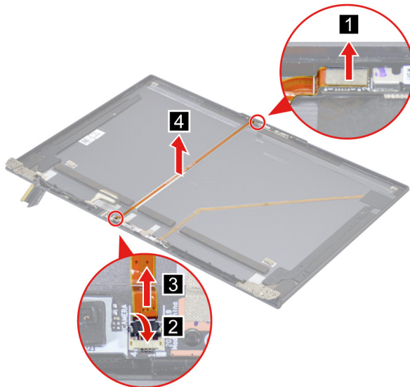
Figure 45. Remove the camera cable
