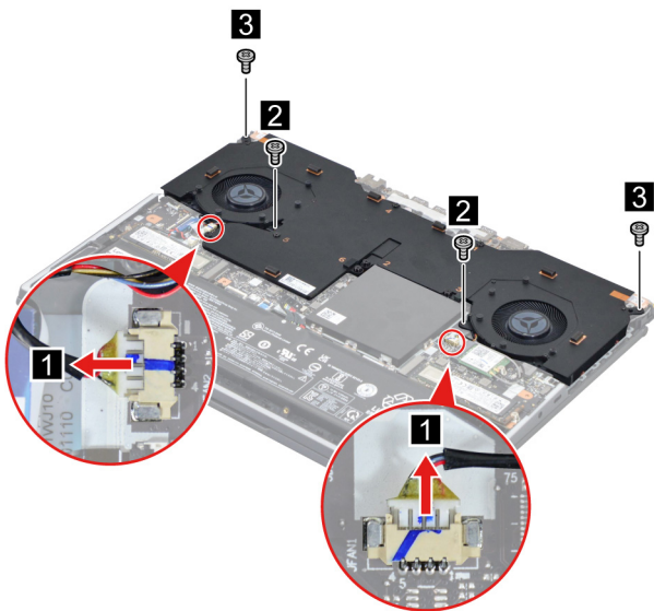
Figure 21. Disconnect the thermal module cable and remove four screws
