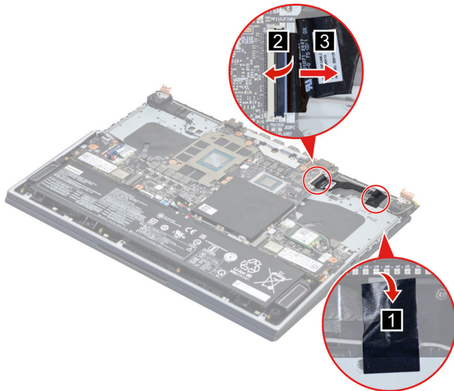
Figure 31. Disconnect the EDP cable
