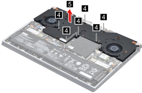
Figure 22. Loosen six screws and then remove the thermal module
