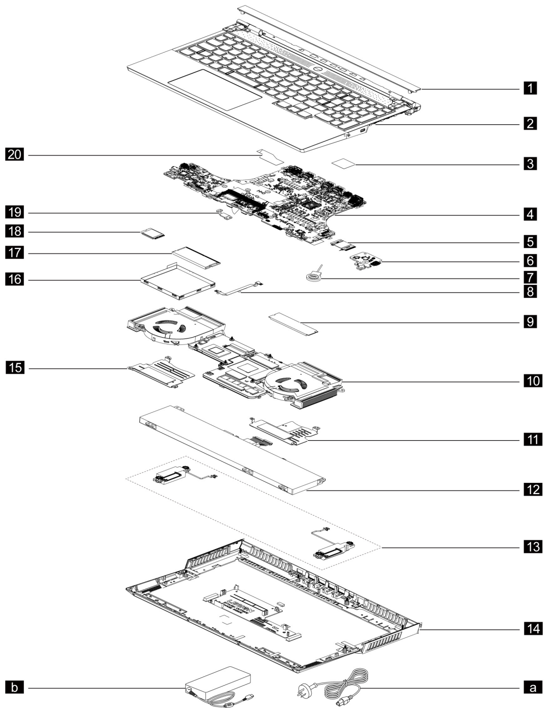
Figure 1. Lenovo Legion 7 (16", 6) exploded view
