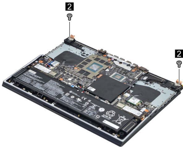
Figure 29. Remove two screws
