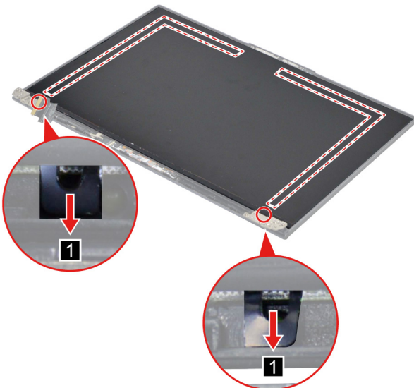
Figure 39. Remove the removable tape
