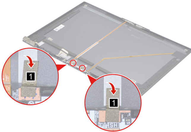
Figure 41. Remove the microphone board conductive tape
