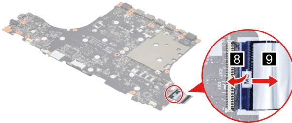
Figure 27. Remove the I/O board cable
