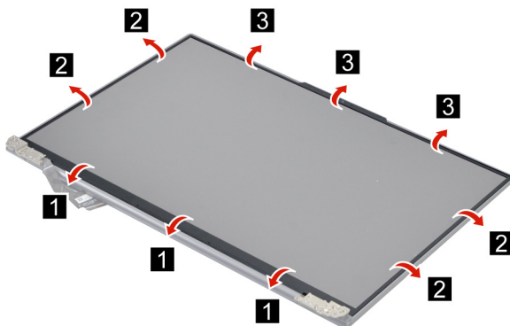
Figure 36. Remove the LCD bezel
