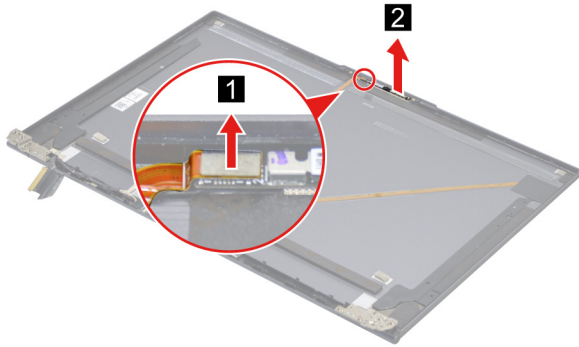
Figure 46. Remove the camera
