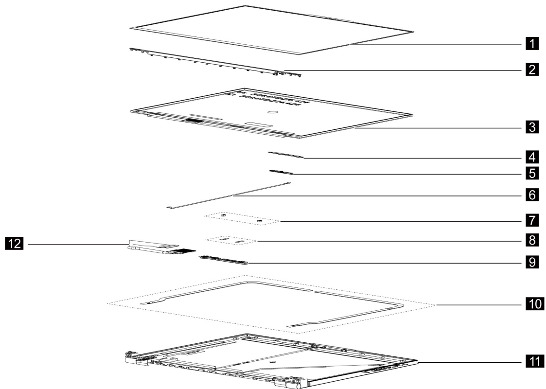
Figure 2. Lenovo Legion 7 (16", 6) LCD module — exploded view
