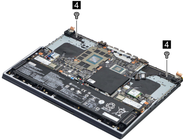
Figure 32. Remove two screws
