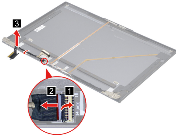
Figure 43. Remove the EDP cable
