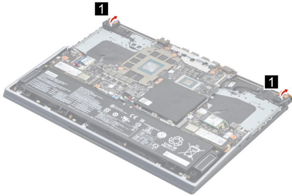
Figure 28. Peel off the antenna tape
