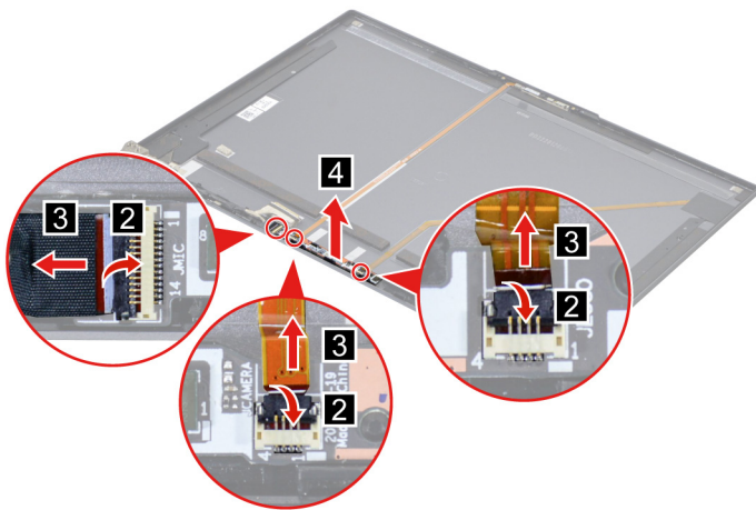
Figure 42. Remove the microphone board
