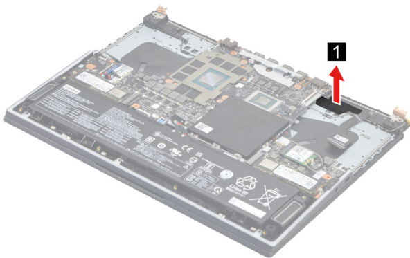
Figure 35. Remove the C cover EDP conductive tape
