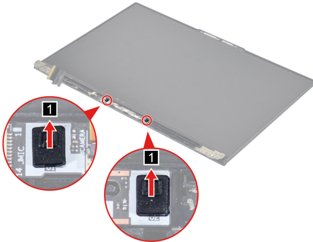
Figure 38. Remove the microphone rubbers
