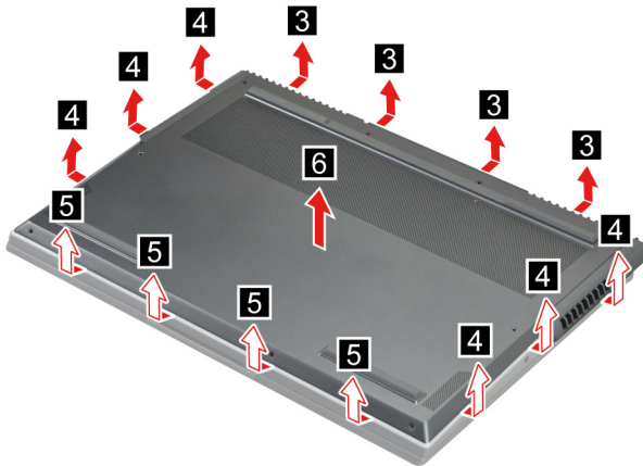
Figure 4. Pry up the latches and then remove the lower case
