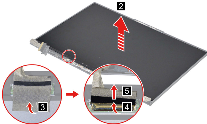
Figure 40. Disconnect the EDP cable and remove the LCD panel
