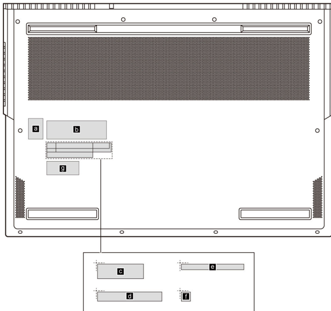
Figure 47. Label layout on the back side of the base cover
