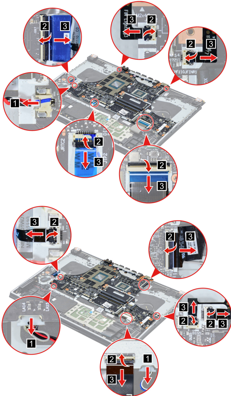
Figure 25. Disconnect cables connected to the system board
