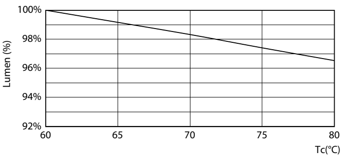
LEDtube MAS 1 15,5W 60K LumenVsTc-LMP
