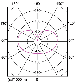
LEDbulb SSW A60 7,5W E27 827 FR-LDD
