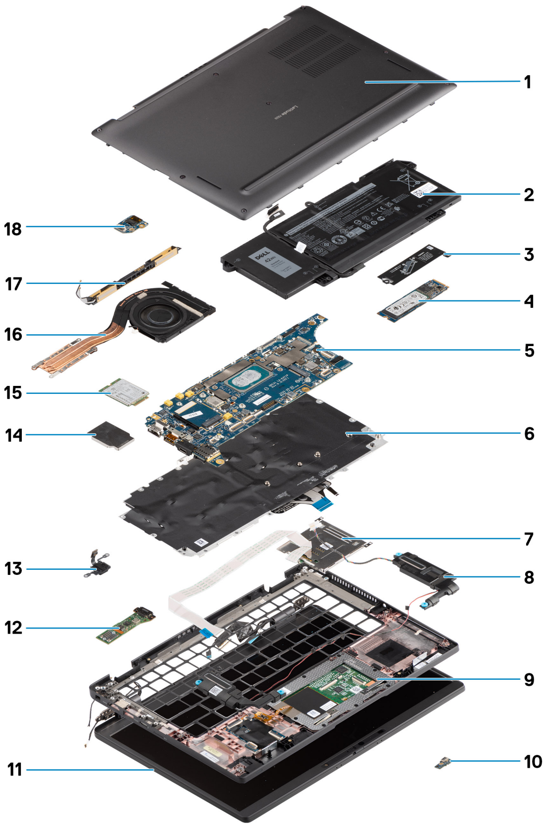
1. Base cover
