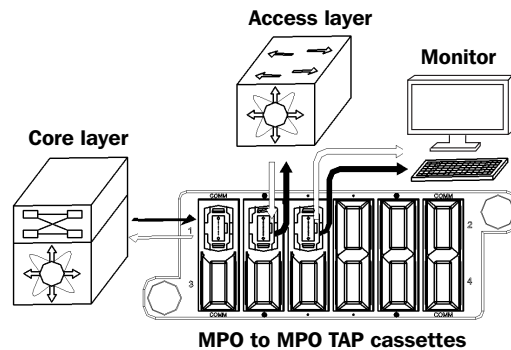
MPO to MPO TAP cassettes
