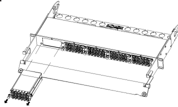
Step 2. Inserting/removing TAP cassettes into panel.
