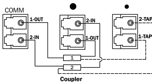
LC to LC TAP port mapping
