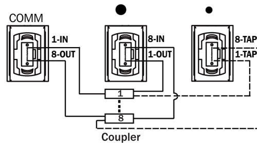
MPO to MPO TAP port mapping
