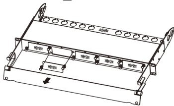
Step 1. Inserting/removing blank plate.
