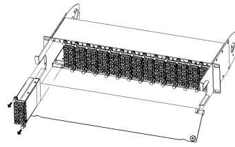
Step 2. Inserting/removing TAP cassettes into panel.
