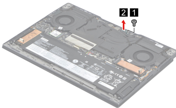
Figure 12. Remove one screw and then remove the DC-in bracket
