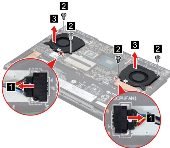
Figure 17. Remove four screws and remove the fans
