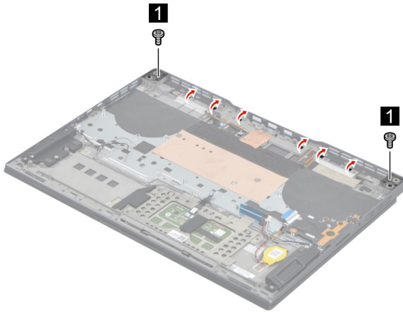
Figure 30. Remove two screws and open the latches
