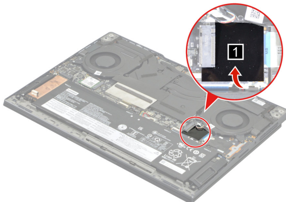
Figure 11. Peel off the SSD mylar
