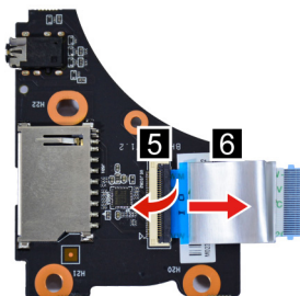
Figure 21. Separate the USB board cable from the USB board
