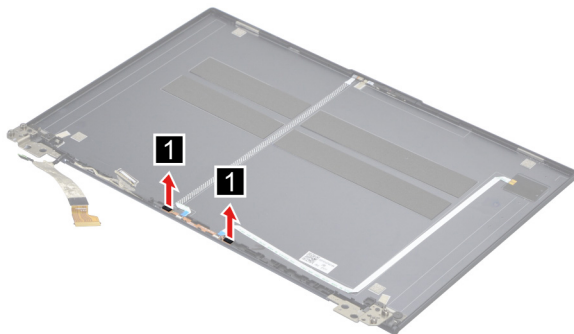
Figure 43. Remove the microphone rubbers
