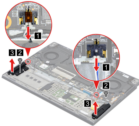
Figure 23. Remove the speakers
