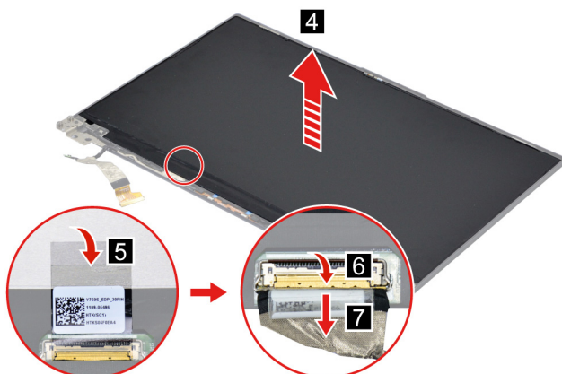
Figure 39. Remove the LCD panel
