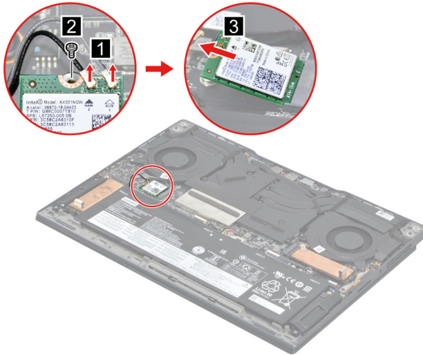
Figure 10. Remove the Wi-Fi card
