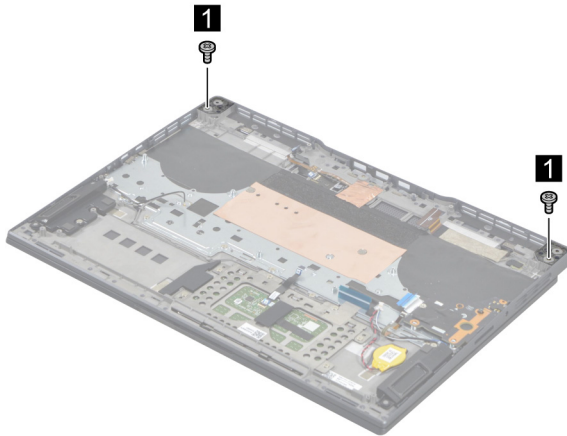
Figure 32. Remove two screws
