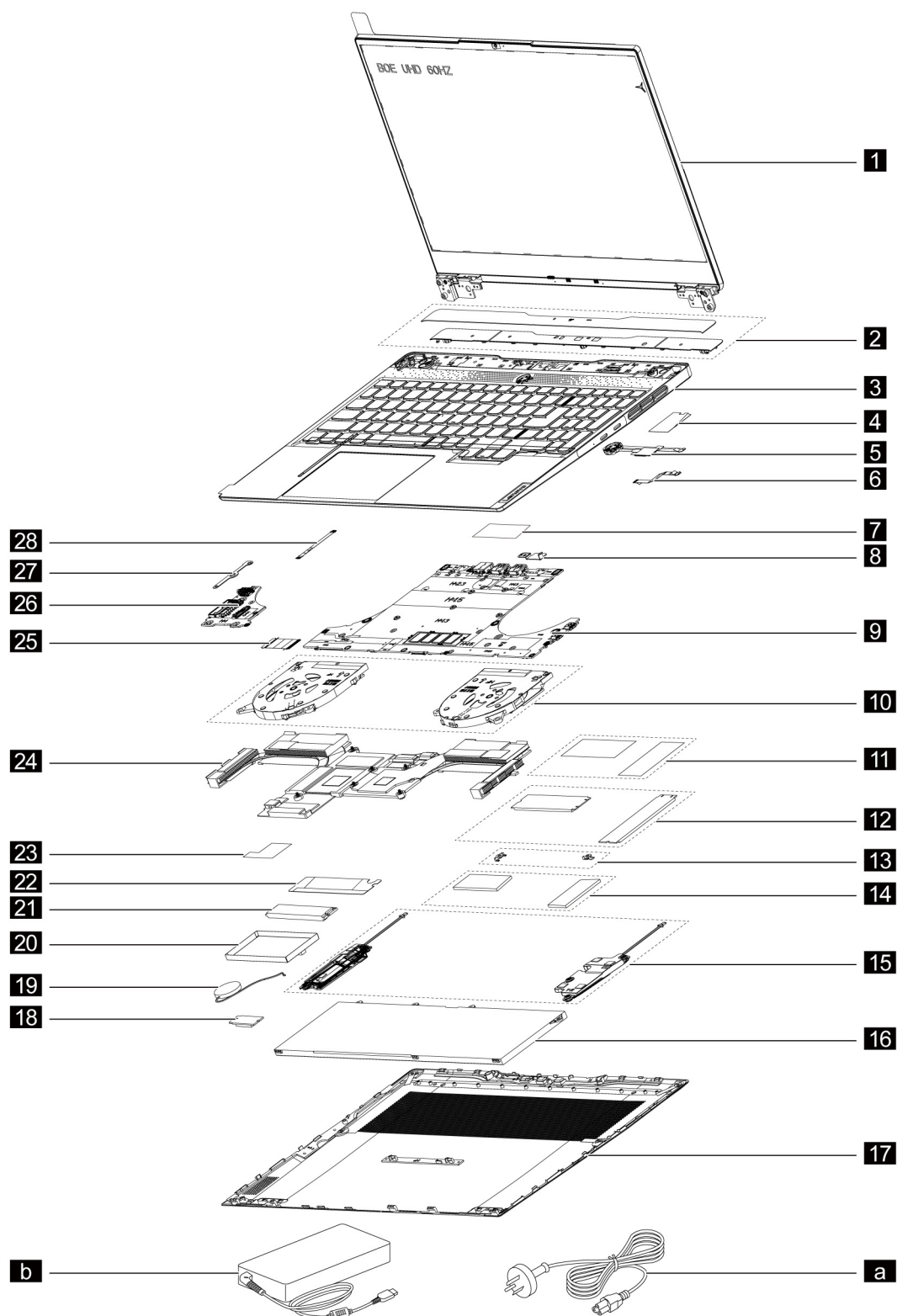
Figure 1. Legion S7 15ACH6 and Lenovo Legion S7 15ACH6 exploded view
