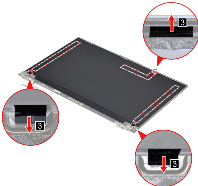
Figure 38. Remove the three pieces of removable tape with tweezers
