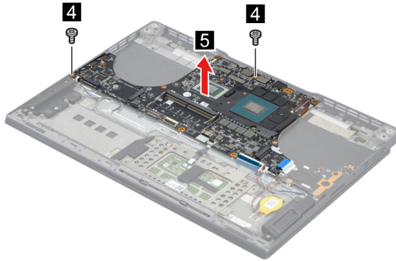
Figure 26. Remove two screws and then remove the system board
