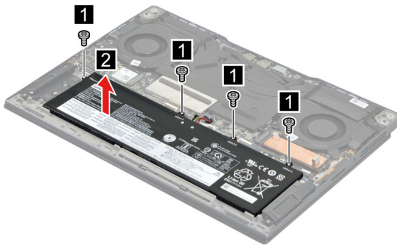
Figure 9. Remove four screws and remove the battery pack
