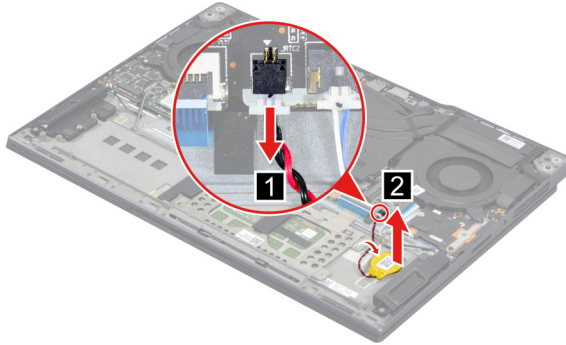
Figure 22. Remove the CMOS battery
