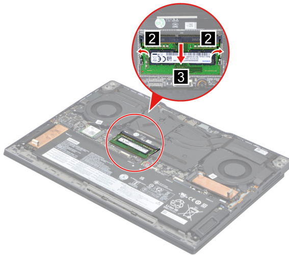
Figure 15. Remove the memory module
