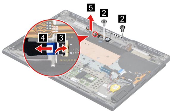
Figure 29. Remove the fingerprint board
