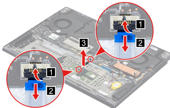
Figure 24. Remove the touchpad cable
