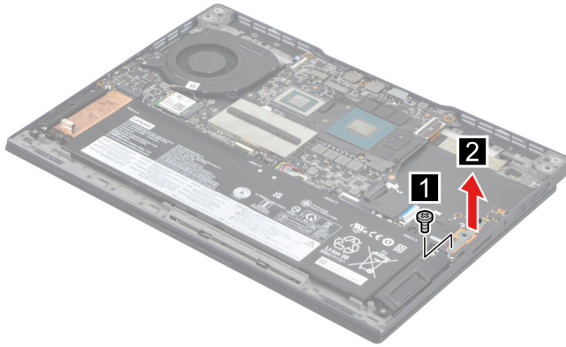
Figure 18. Remove the SSD bracket
