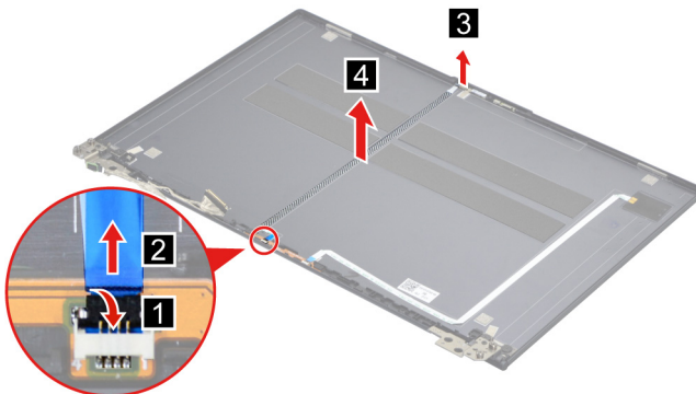
Figure 41. Remove the camera cable
