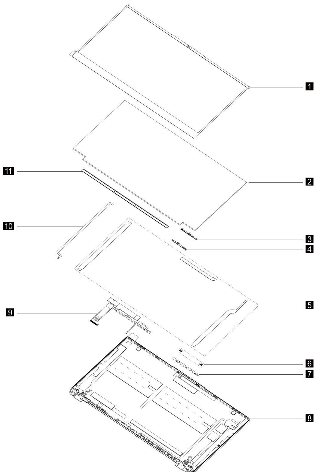
Figure 2. Legion S7 15ACH6 and Lenovo Legion S7 15ACH6 LCD module- exploded view
