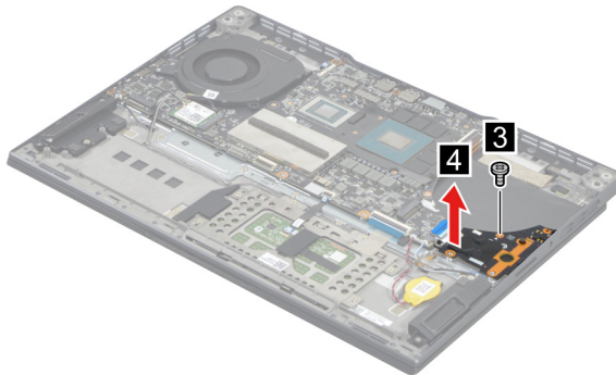
Figure 20. Remove one screw and then remove the USB board with cable
