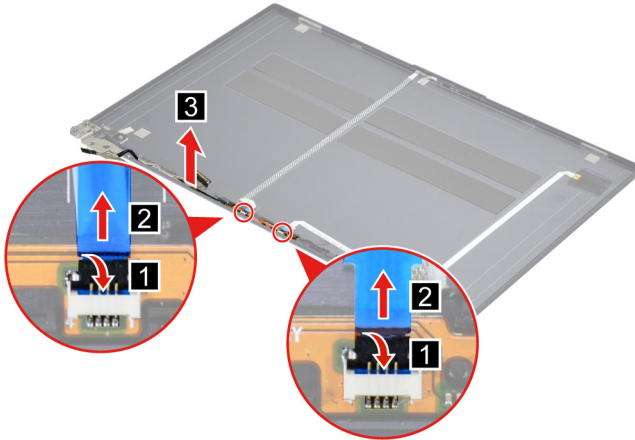
Figure 44. Remove the microphone board and the EDP cable
