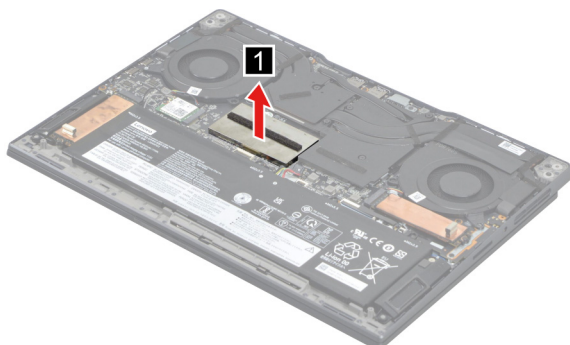
Figure 14. Remove the memory module shielding
