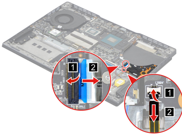
Figure 19. Disconnect the cable connected to the USB board and disconnect the USB board cabled
