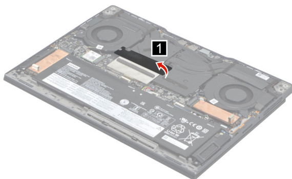
Figure 13. Peel off the memory module mylar
