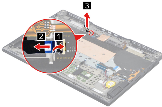
Figure 27. Remove the fingerprint board cable
