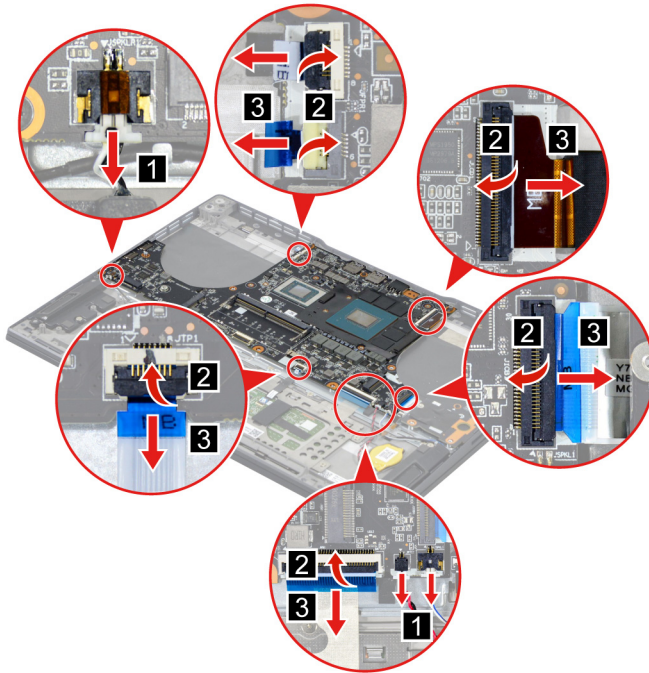
Figure 25. Disconnect cables connected to the system board
