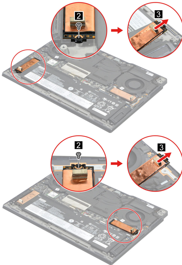
Figure 6. Remove two screws and remove the SSD module
