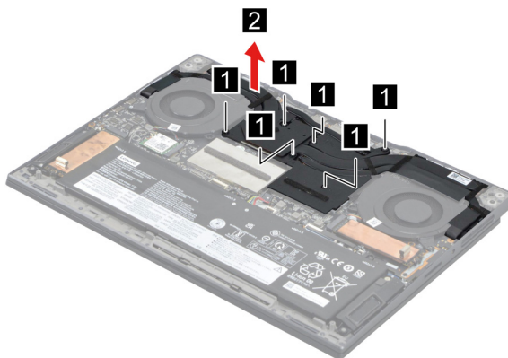
Figure 16. Loosen six screws and then remove the heat sink
