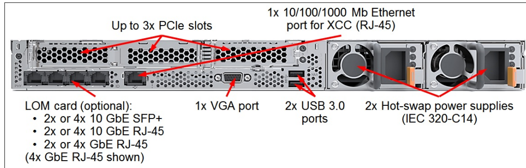
Figure 5. Rear view of the SR630
