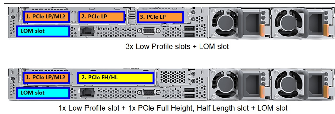
Figure 8. Slot locations
