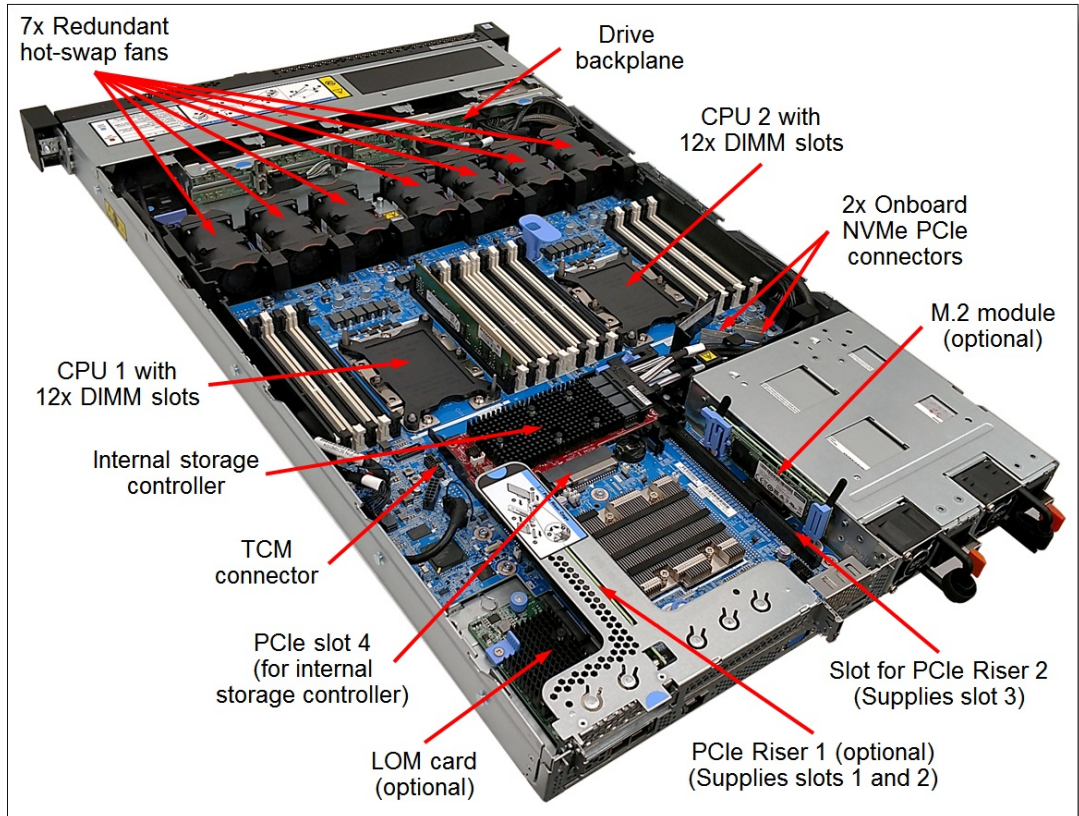
Figure 6. Internal view of the SR630
