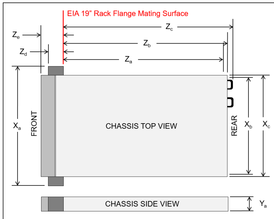
Figure 9. Server dimensions
