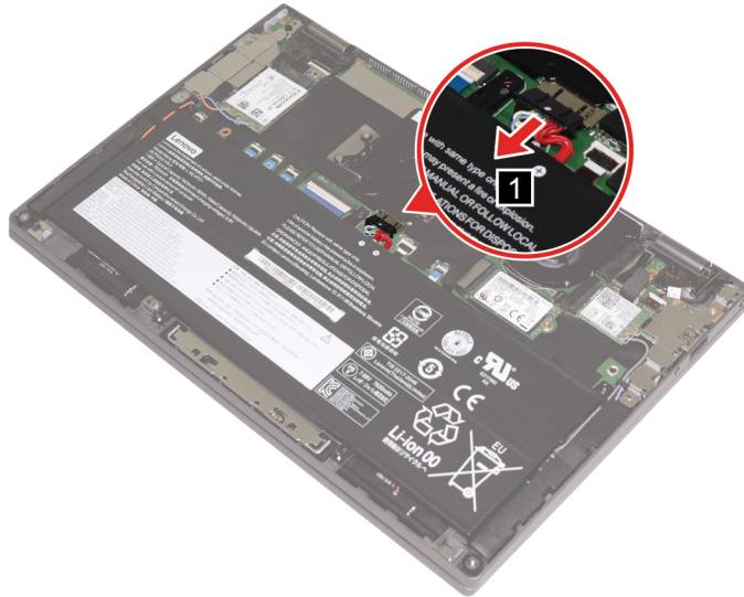
Figure 7. Disconnect the battery cables
