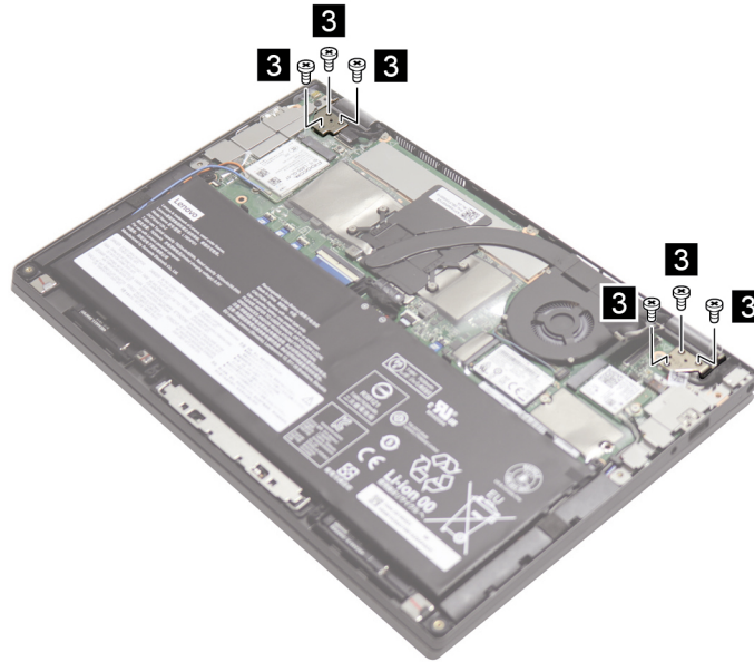
Figure 24. Remove six screws
