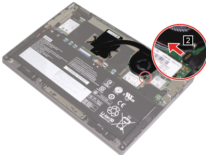
Figure 8. Disconnect the thermal module cable from the system board
