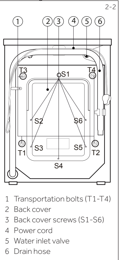
Rear side (Fig. 2-2):
