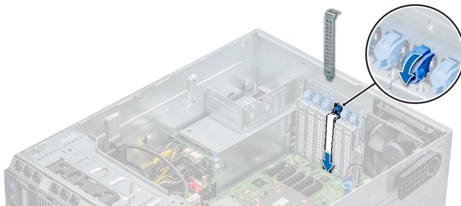
Figure 62. Installation du support de recouvrement
