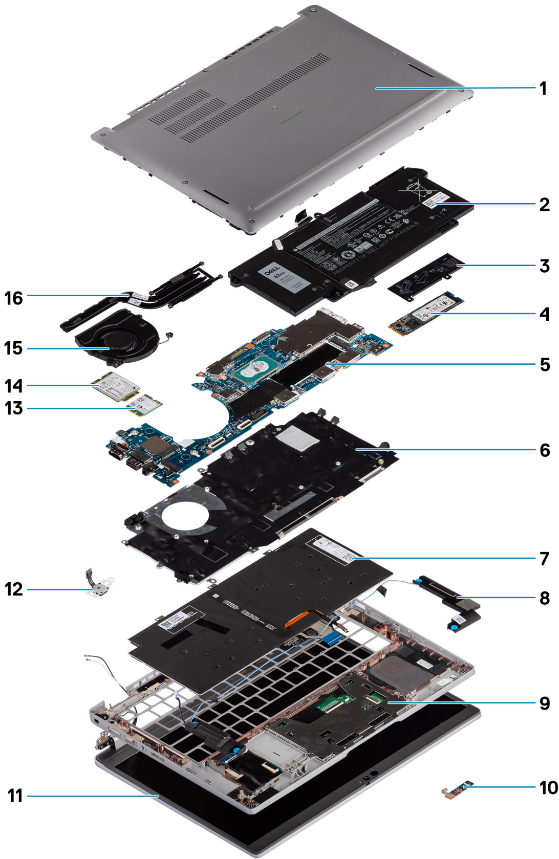
1. Base cover
