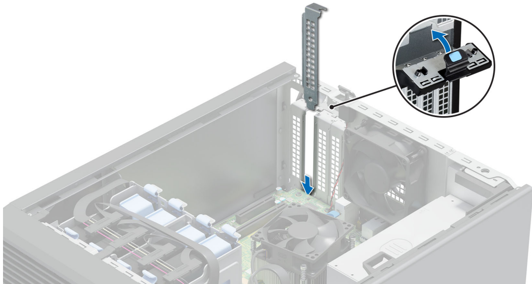
Figure 38. Installation de la plaque de recouvrement
