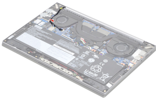
Figure 11. Release the antenna cable from the cable guide
