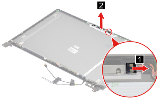
Figure 44. Disconnect the camera cable from the camera board and remove the camera
