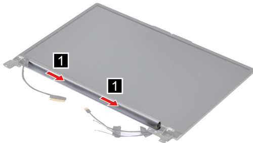
Figure 35. Remove the hinge cover
