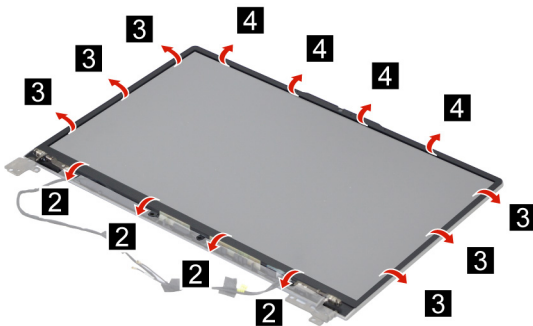
Figure 38. Remove the LCD bezel
