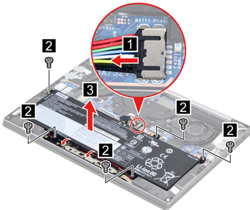
Figure 5. Remove five screws and remove the battery pack
