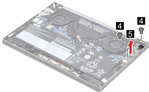
Figure 18. Remove two screws and remove the I/O bracket (left)
