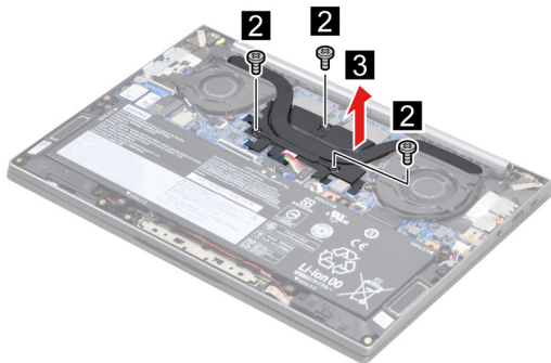
Figure 7. Remove three screws and then remove the heat sink
