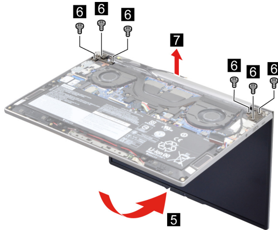
Figure 34. Remove six screws and remove the LCD unit
