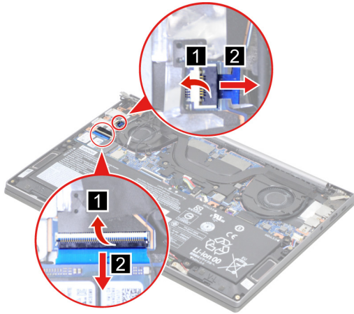
Figure 19. Disconnect the I/O board cable and the fingerprint board cable from the I/O board
