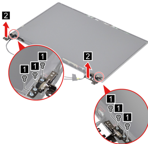
Figure 40. Remove six screws and remove the hinges
