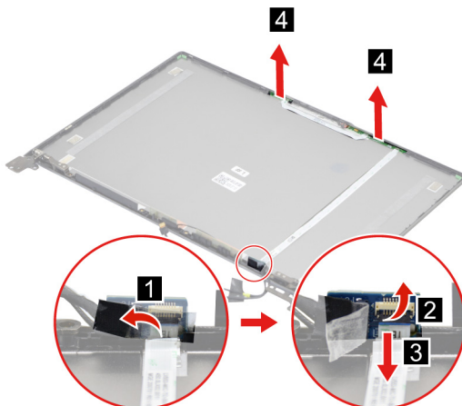
Figure 45. Remove the microphone board with cables
