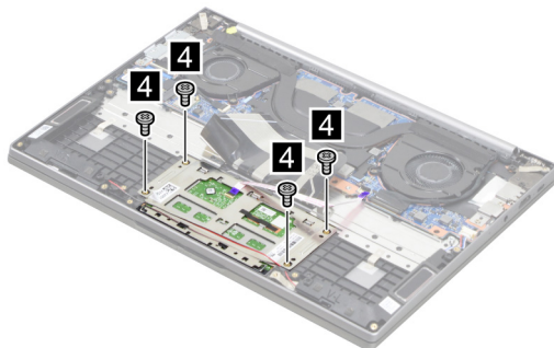
Figure 30. Remove four screws
