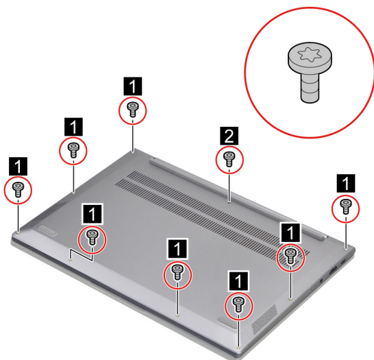
Figure 3. Remove nine screws
