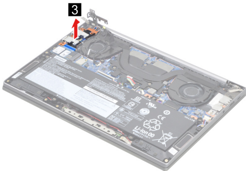
Figure 20. Remove the I/O board
