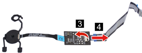
Figure 23. Separate the fingerprint board cable from the fingerprint board
