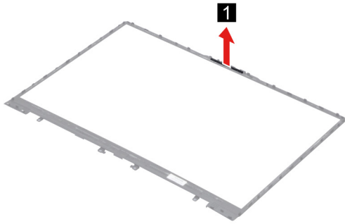
Figure 39. Remove the camera privacy shutter
