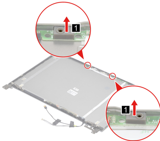
Figure 43. Remove the microphone rubbers
