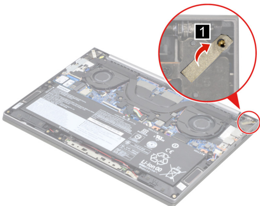
Figure 16. Peel off the tape
