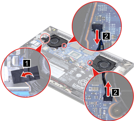
Figure 14. Peel off the tape and disconnect the fan cables from the system board
