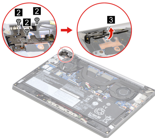
Figure 12. Remove three screws and then open the hinge
