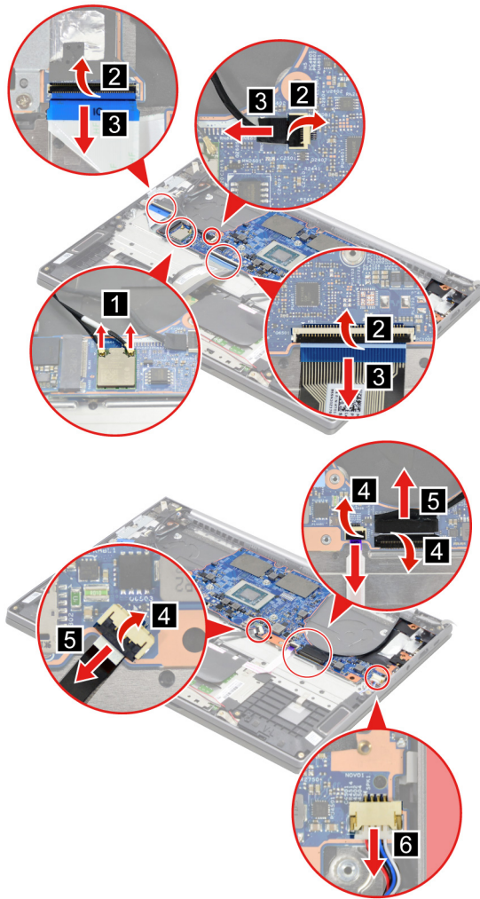
Figure 25. Disconnect cables connected to the system board
