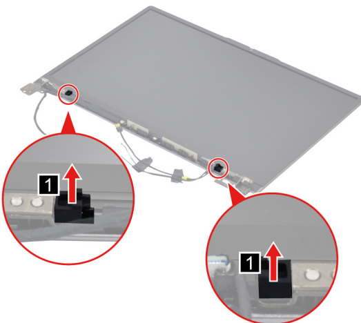
Figure 36. Remove the hinge rubbers
