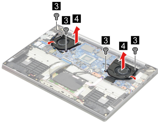
Figure 15. Remove four screws and then remove the fans
