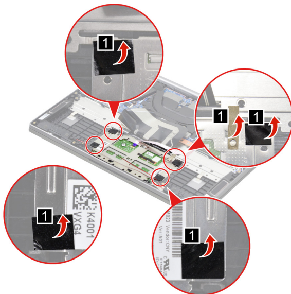
Figure 28. Peel off the pieces of tape
