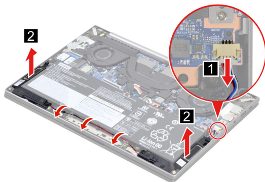
Figure 24. Remove the speakers
