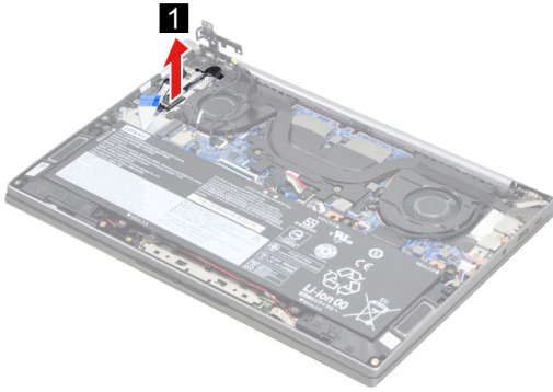
Figure 21. Remove the fingerprint board module
