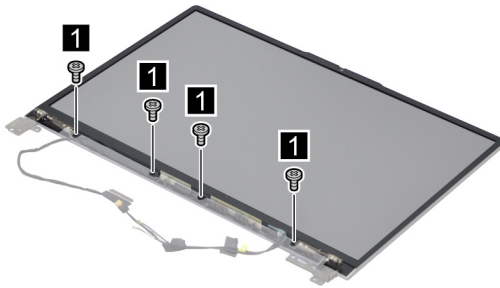
Figure 37. Remove four screws
