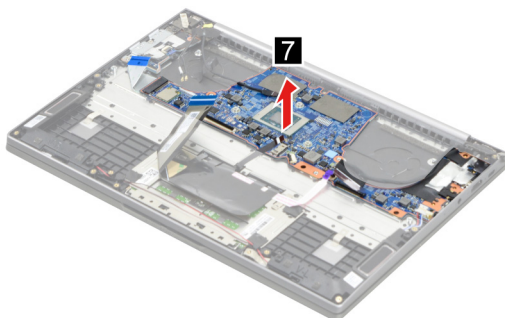
Figure 26. Remove the system board and the I/O board cable
