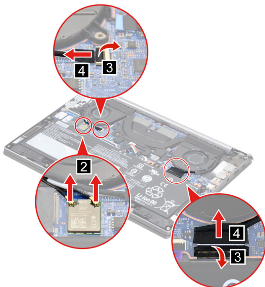
Figure 33. Detach the antenna cable connectors, disconnect the trans board cable and the EDP cable from the system board
