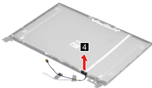
Figure 47. Remove the trans board with cable
