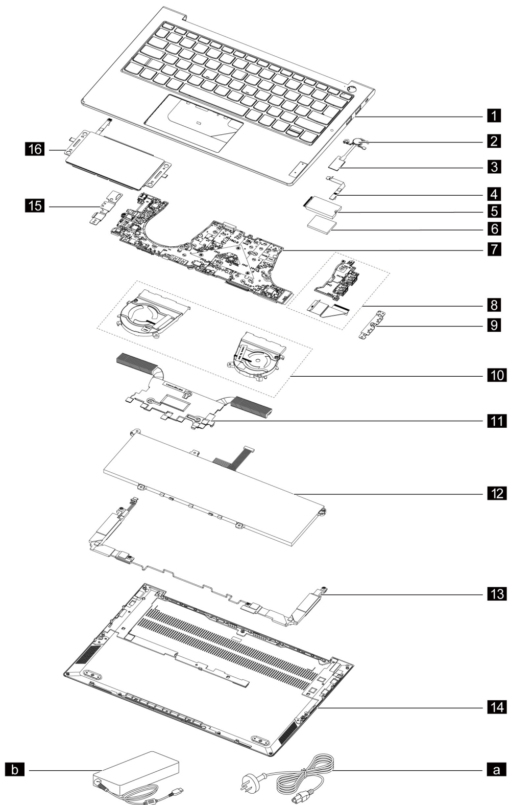
Figure 1. ThinkBook 13s G3 ACN and ThinkBook 14s G3 ACN exploded view
