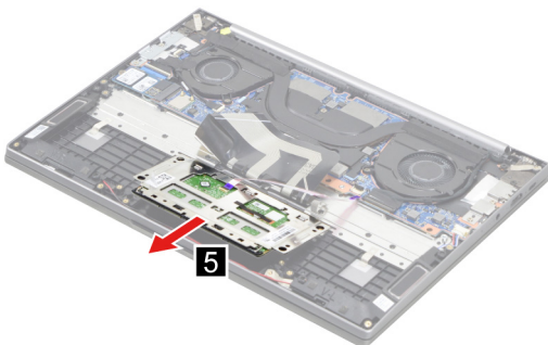
Figure 31. Remove the touchpad with cable
