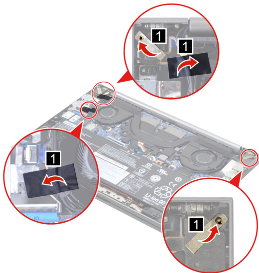
Figure 32. Peel off the pieces of tape
