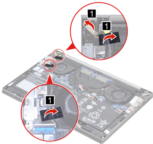
Figure 10. Peel off the pieces of tape
