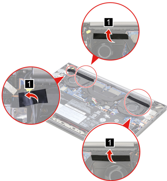
Figure 6. Peel off the pieces of tape
