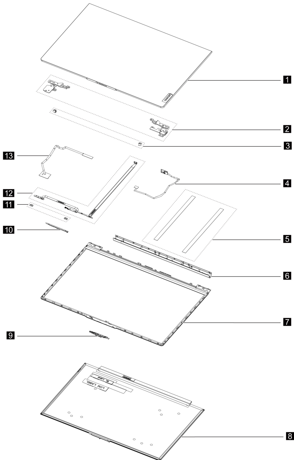
Figure 2. ThinkBook 13s G3 ACN and ThinkBook 14s G3 ACN LCD unit - exploded view
