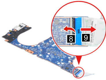
Figure 27. Separate the I/O board cable from the system board
