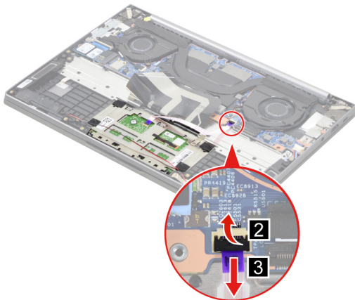
Figure 29. Disconnect the touchpad cable from the system board
