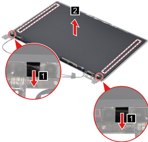
Figure 41. Remove the two pieces of removable tape with tweezers and then remove the LCD panel
