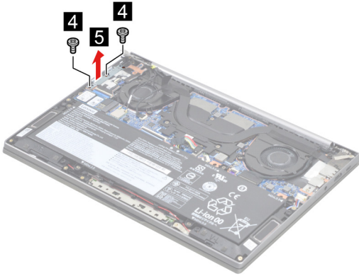
Figure 13. Remove two screws and remove the I/O bracket (right)
