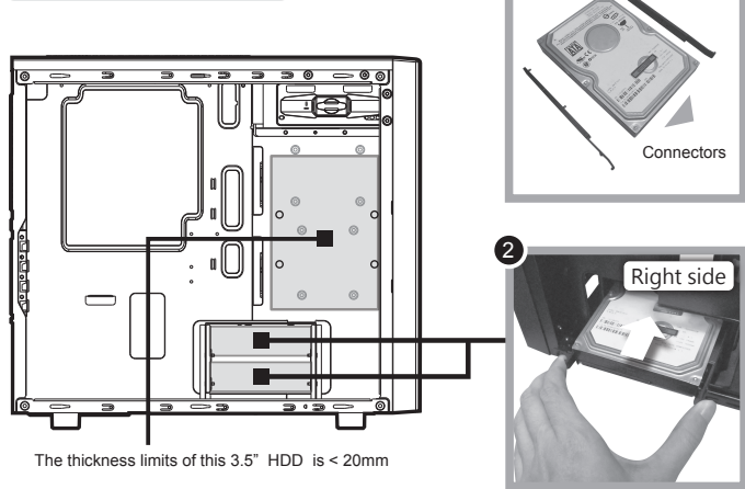
How to install a 3.5" HDD
