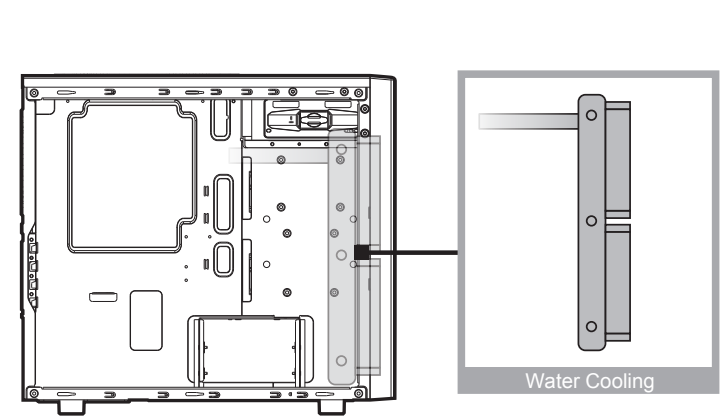
How to install water cooling radiator
