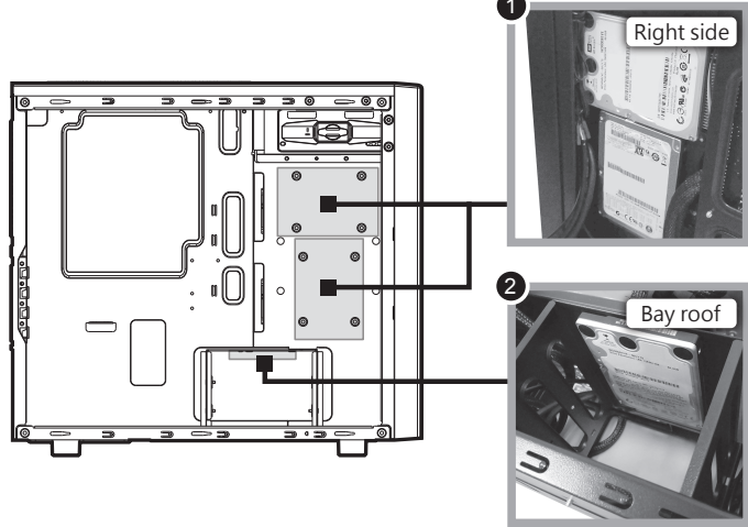
How to install a 2.5" HDD/SSD
