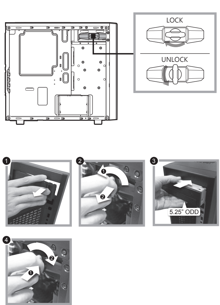
How to install the 5.25" device
