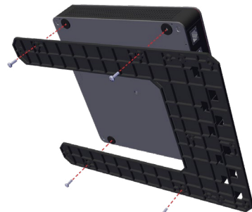
Figure 2 - Bracket Removal
