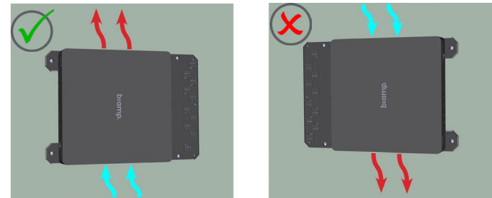
Figure 3 - Proper Airflow
