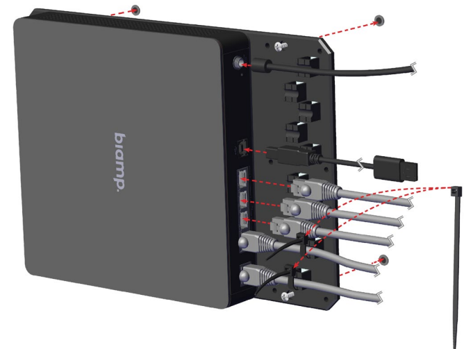
Figure 4 - Devio SCX Wall Installation with Cable Management Tray
