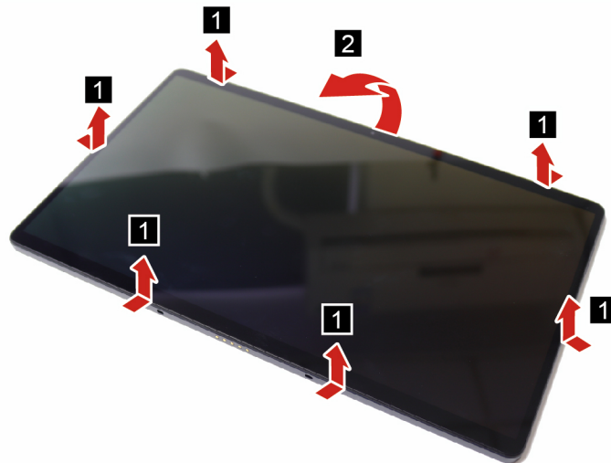
Figure 2. Lift the LCD module
