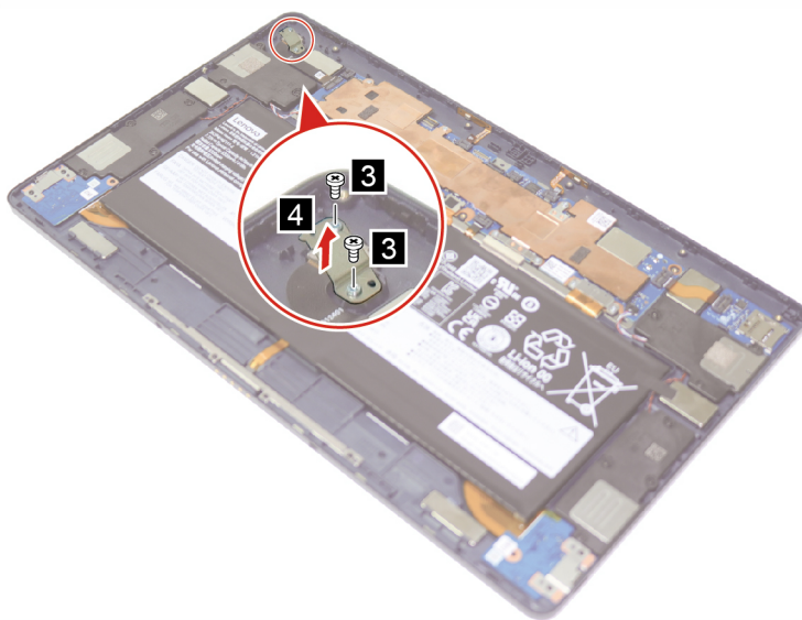
Figure 23. Remove the rear-facing camera bracket
