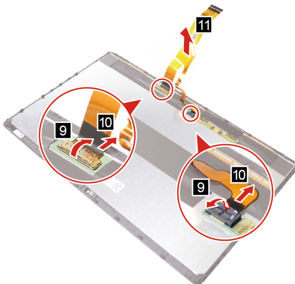
Figure 5. Disconnect the EDP cable
