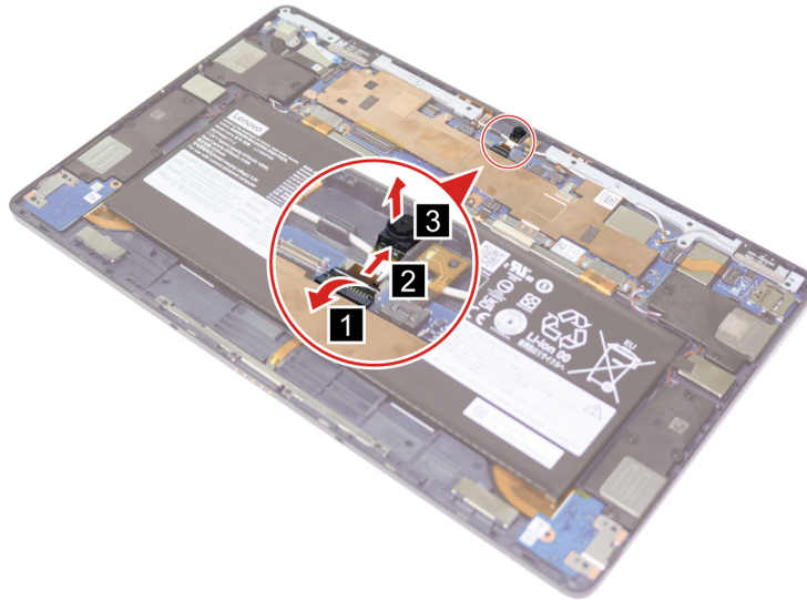
Figure 15. Remove the front-facing camera
