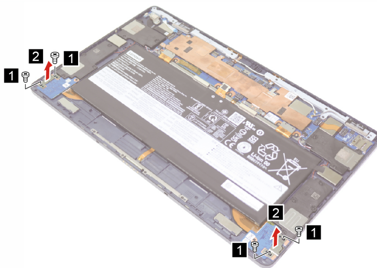
Figure 10. Remove four screws and the I/O board cable brackets
