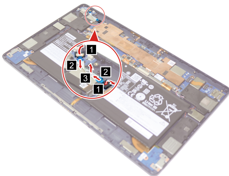
Figure 20. Disconnect and remove the power volume board cable
