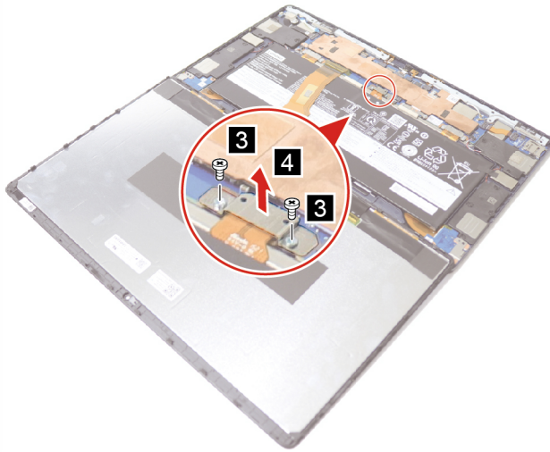
Figure 3. Remove two screws and the battery pack cable bracket
