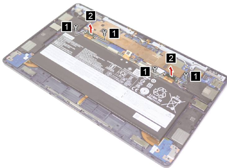
Figure 9. Remove four screws and the I/O board cable brackets
