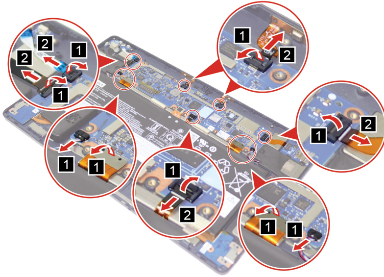
Figure 25. Disconnect cables
