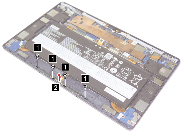
Figure 13. Remove four screws and remove pogo pin bracket
