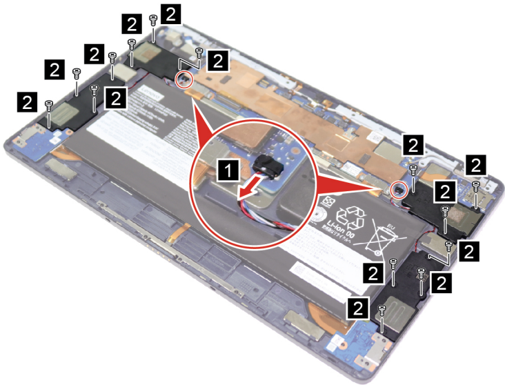
Figure 7. Disconnect cables
