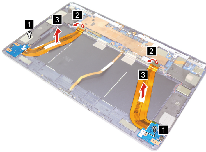
Figure 11. Remove two screws and disconnect cables
