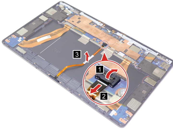
Figure 27. Remove the pogo pin cable
