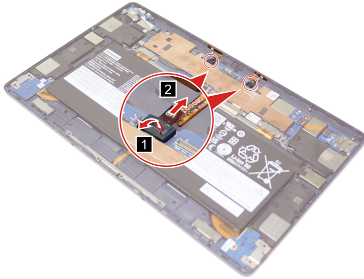
Figure 19. Remove the microphone cables
