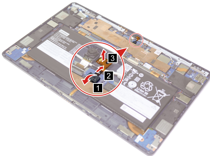
Figure 16. Remove the front-facing camera LED cable
