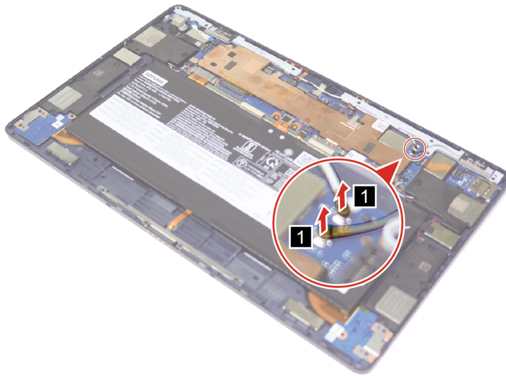
Figure 17. Disconnect the antennas
