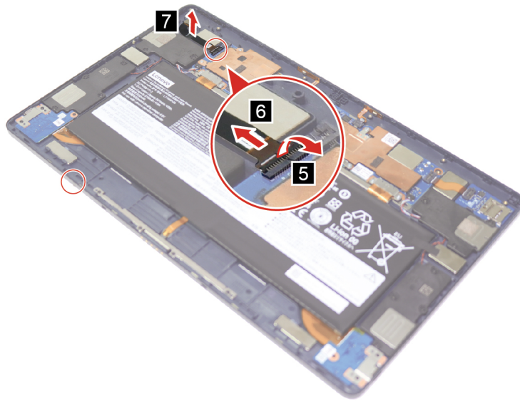
Figure 24. Disconnect and remove the rear-facing camera
