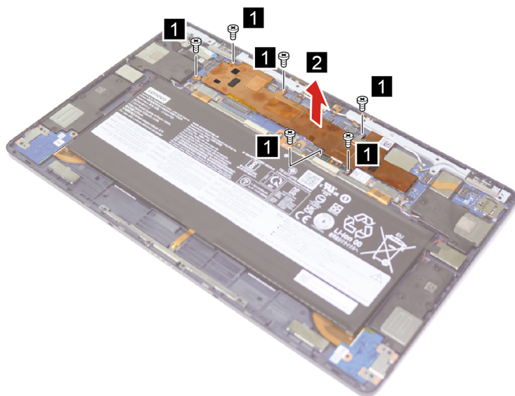
Figure 14. Remove six screws and remove the heat sink
