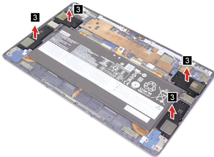
Figure 8. Remove speakers
