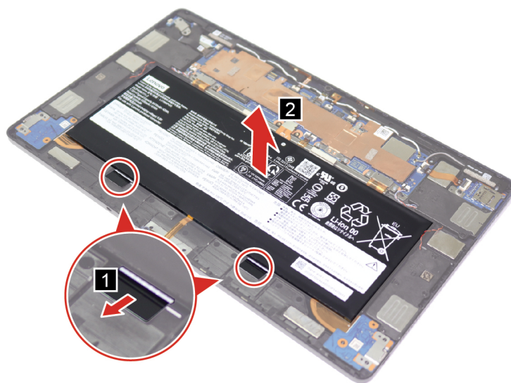
Figure 6. Remove the battery pack
