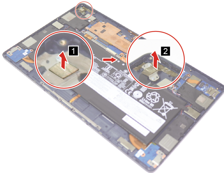
Figure 22. Remove the rear-facing camera sponge and rear-facing camera conductive cloth
