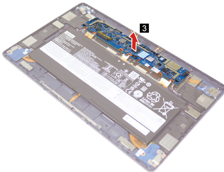
Figure 26. Remove the system board
