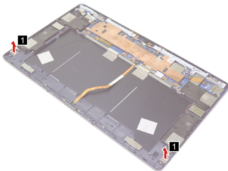
Figure 28. Remove the I/O rubbers
