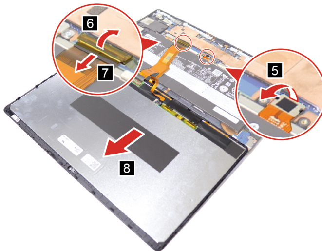
Figure 4. Disconnect cables and remove the LCD module
