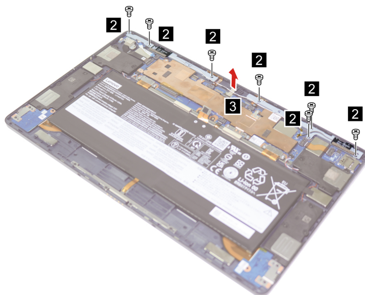
Figure 18. Remove seven screws and remove the antenna module
