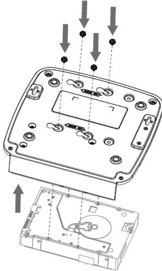
Figure 2-32 Install HDD
