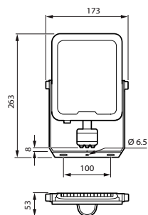
BVP164 LED60/840 PSU 50W SWB MDU CE
