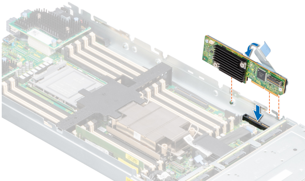
Figure 18. Installation de la Dell HBA350i MX
