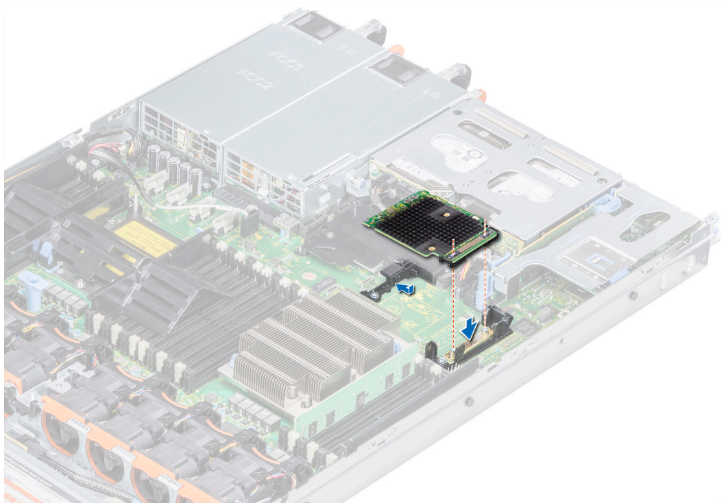
Figure 23. Installation de la Dell HBA350i MM
