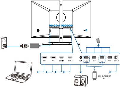
USB hub
